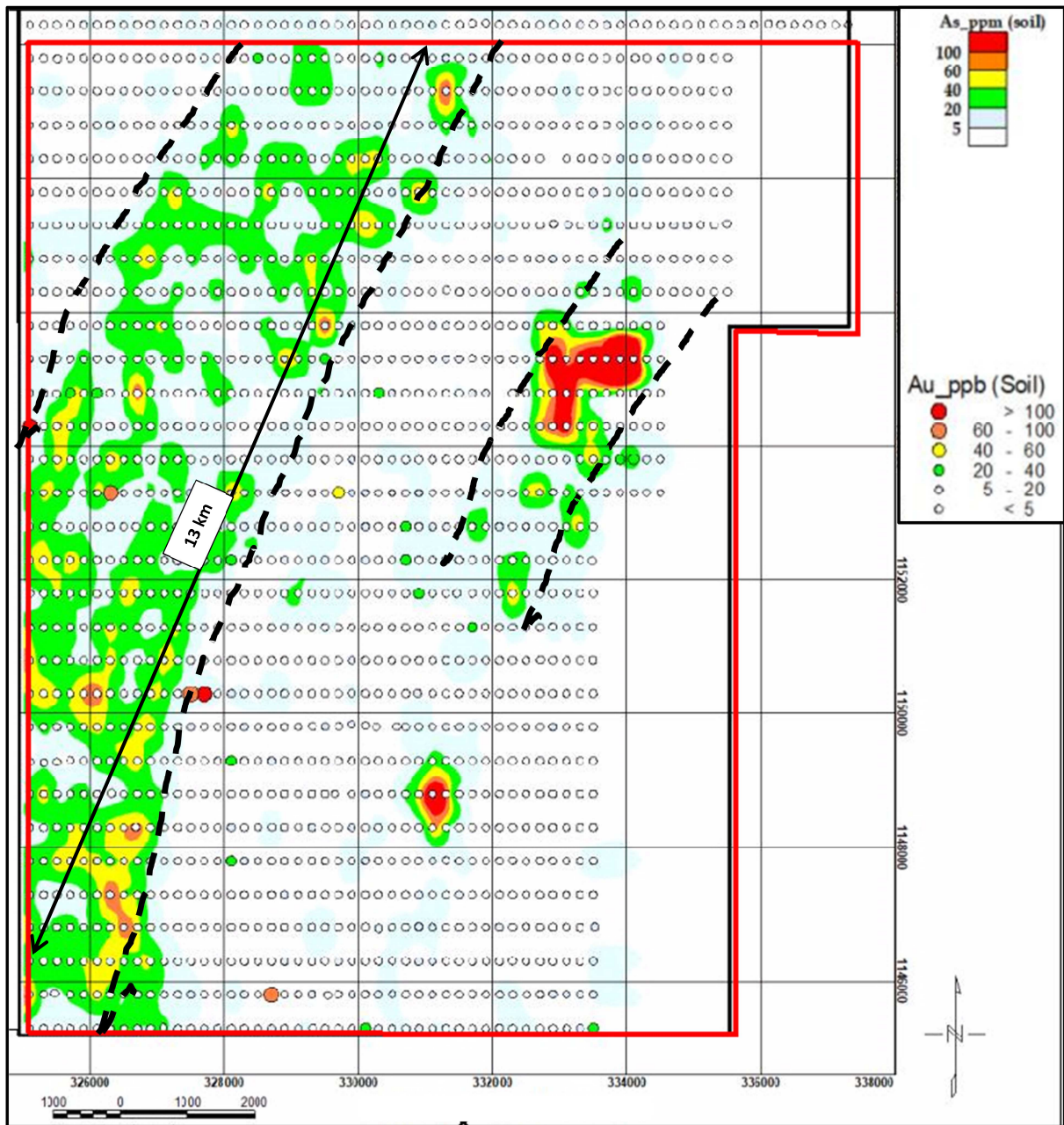
Boulon historical soil geochemistry (Gold and Arsenic) results
