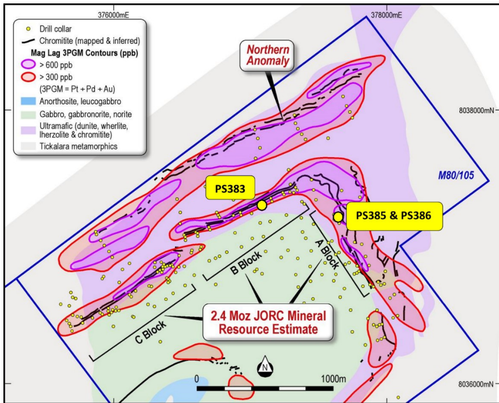
Figure One | Panton Drill Hole Plan
