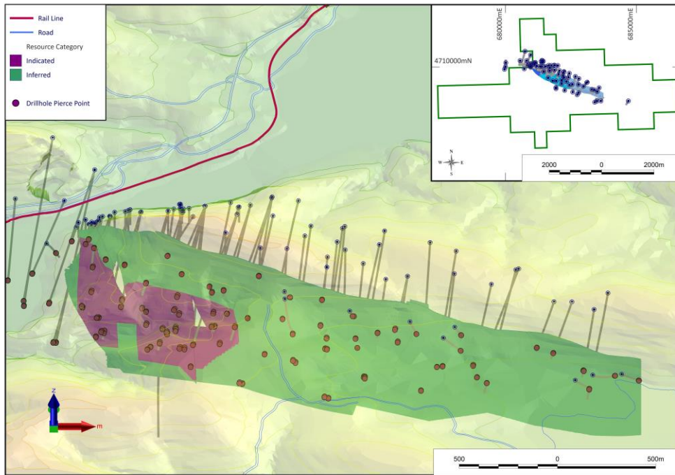
Figure 9 Toral Updated block model looking North
