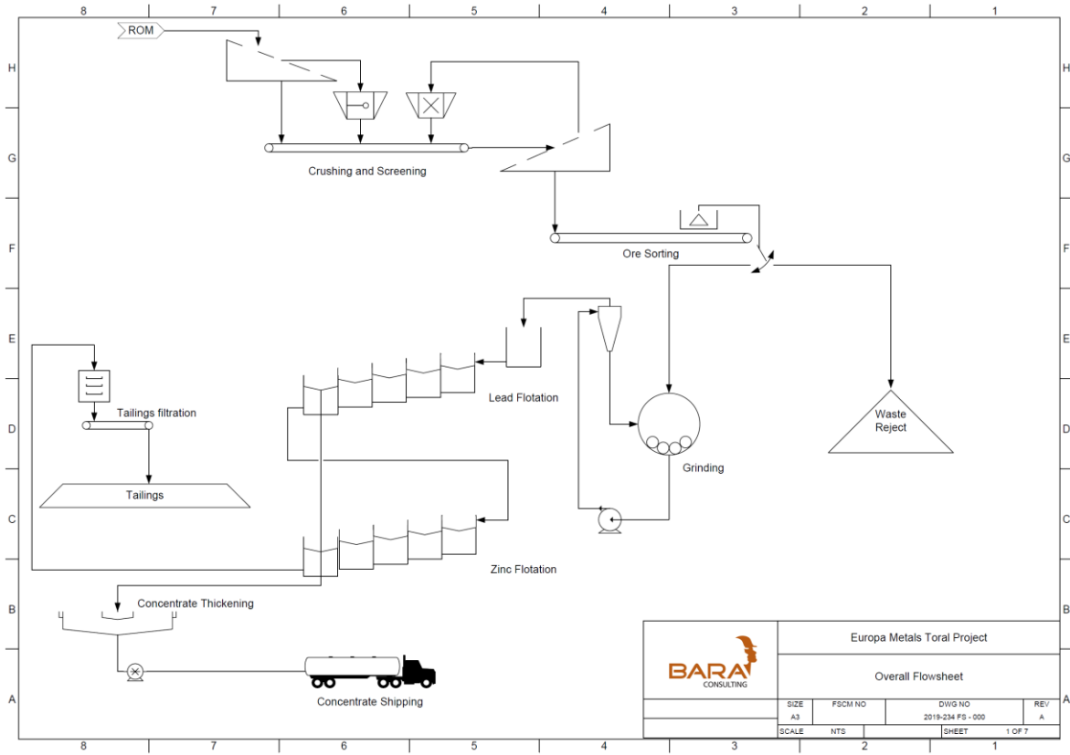
Figure 7 Toral Overall Flowsheet showing Crushing, Sorting, Grinding and Flotation
