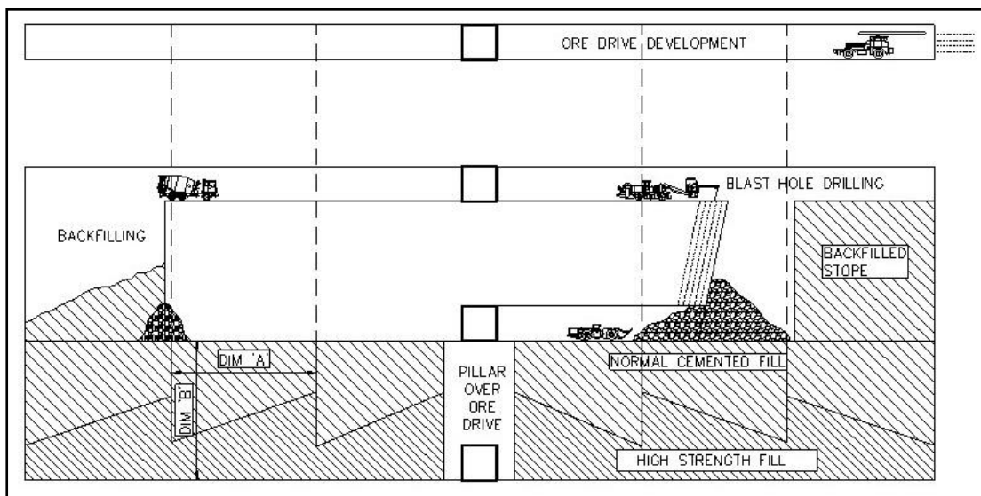
Figure 5 Typical sub-level set of 3 levels showing underhand development sequence, overhand stoping sequence and pillar layout
