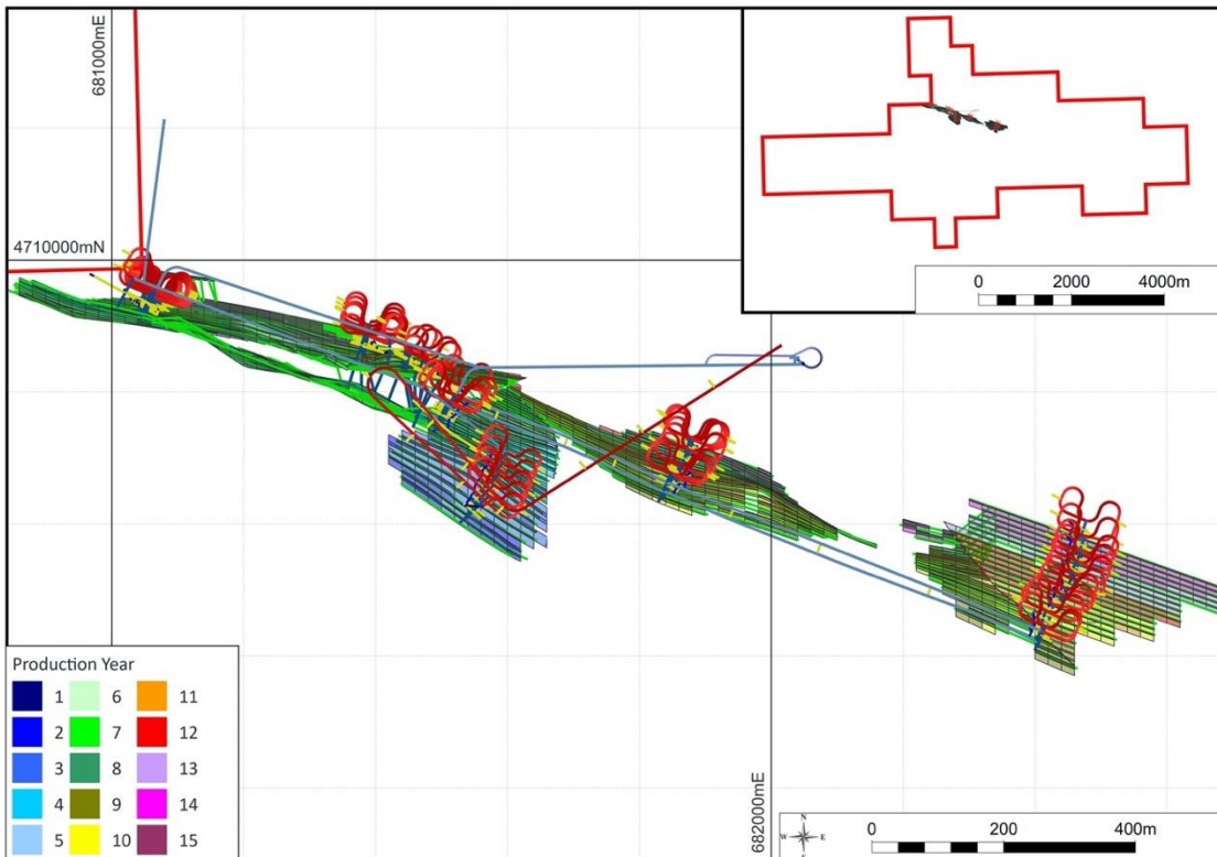
Figure 3 Total Mining plan situated within overall licence area showing under explored Eastern area
