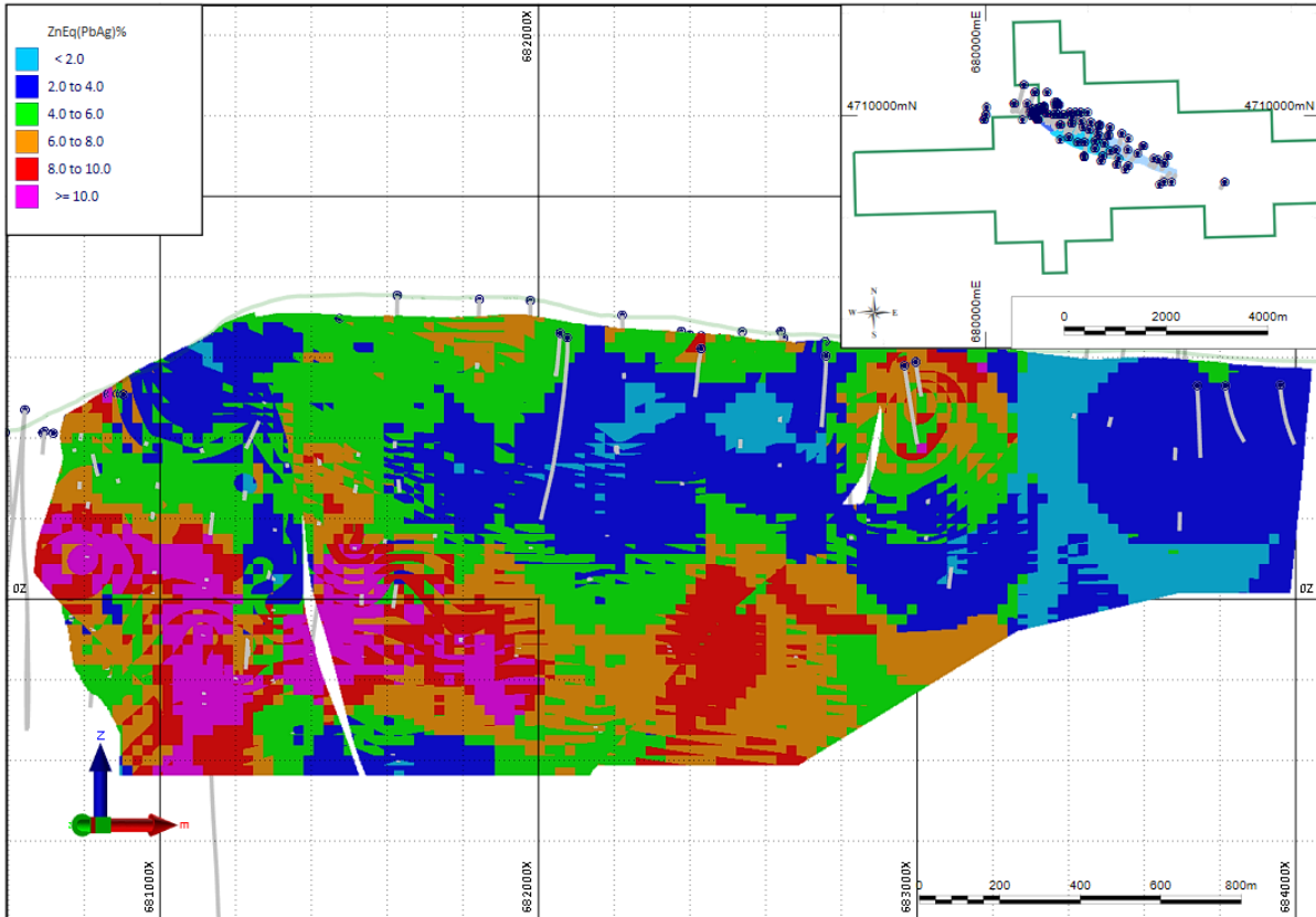
FIGURE 3: AMS' East West 2D Toral block model by grade
