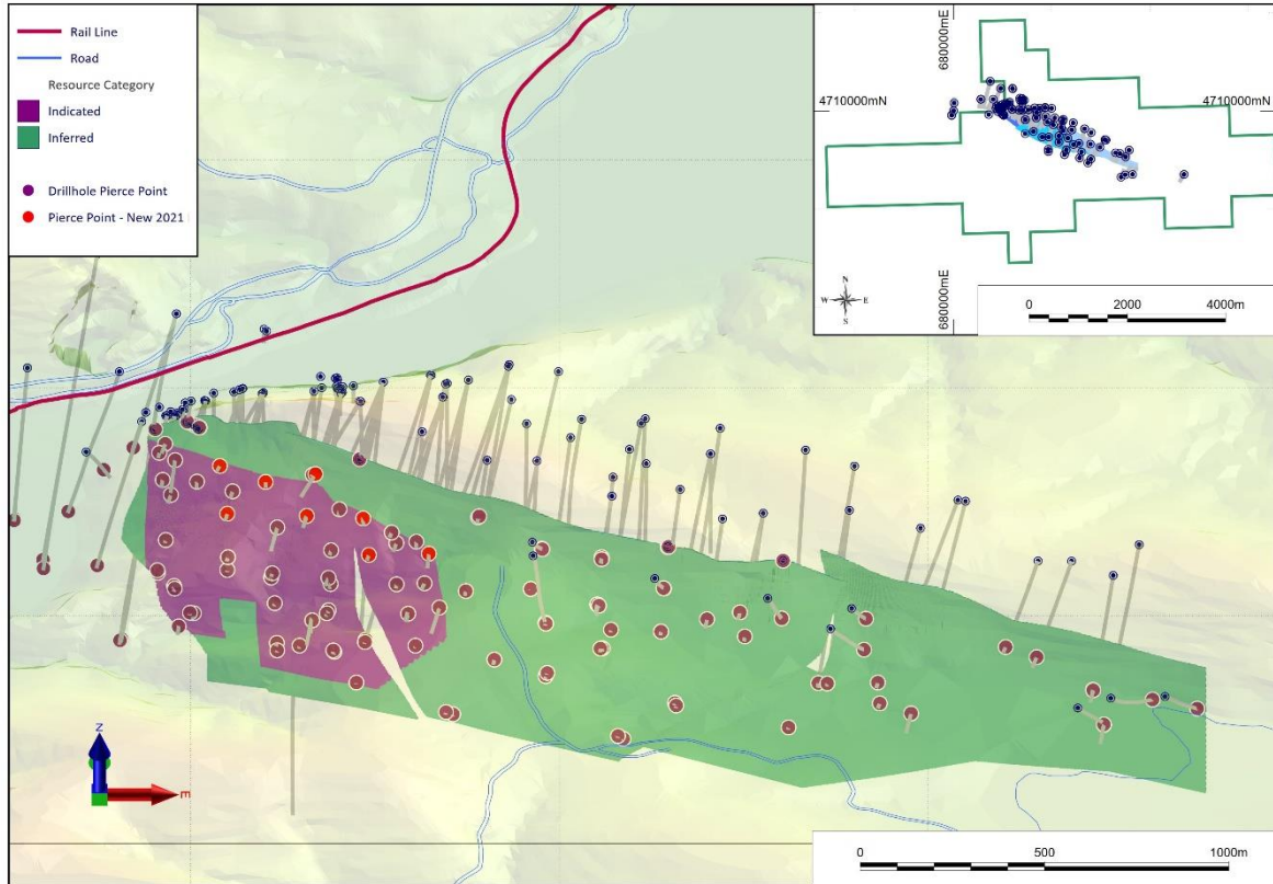
FIGURE 2a: AMS' resource block model for Toral as a 3D view looking north, by resource category, Indicated blocks in purple, Inferred Blocks in green
