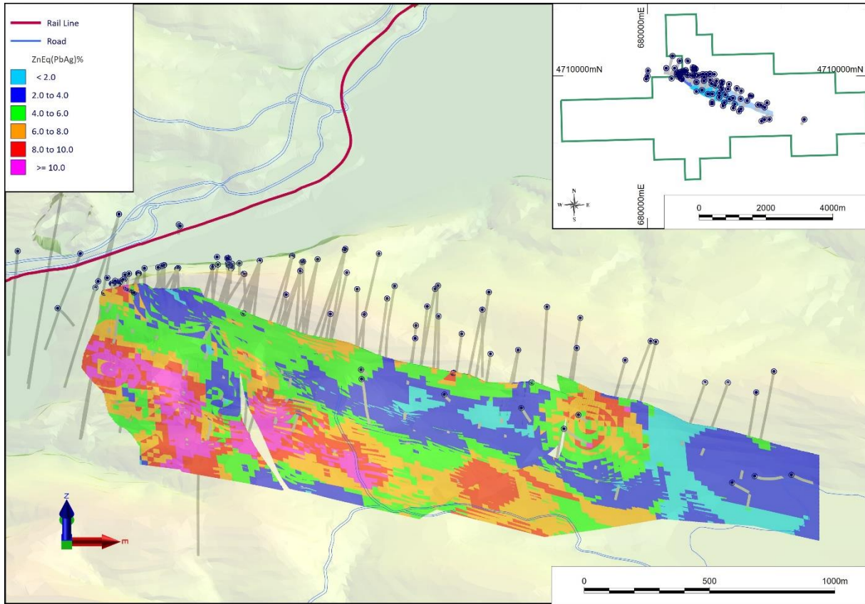
FIGURE 1: AMS' resource block model for Toral as a 3D view looking north, by Zn Equivalent grade
