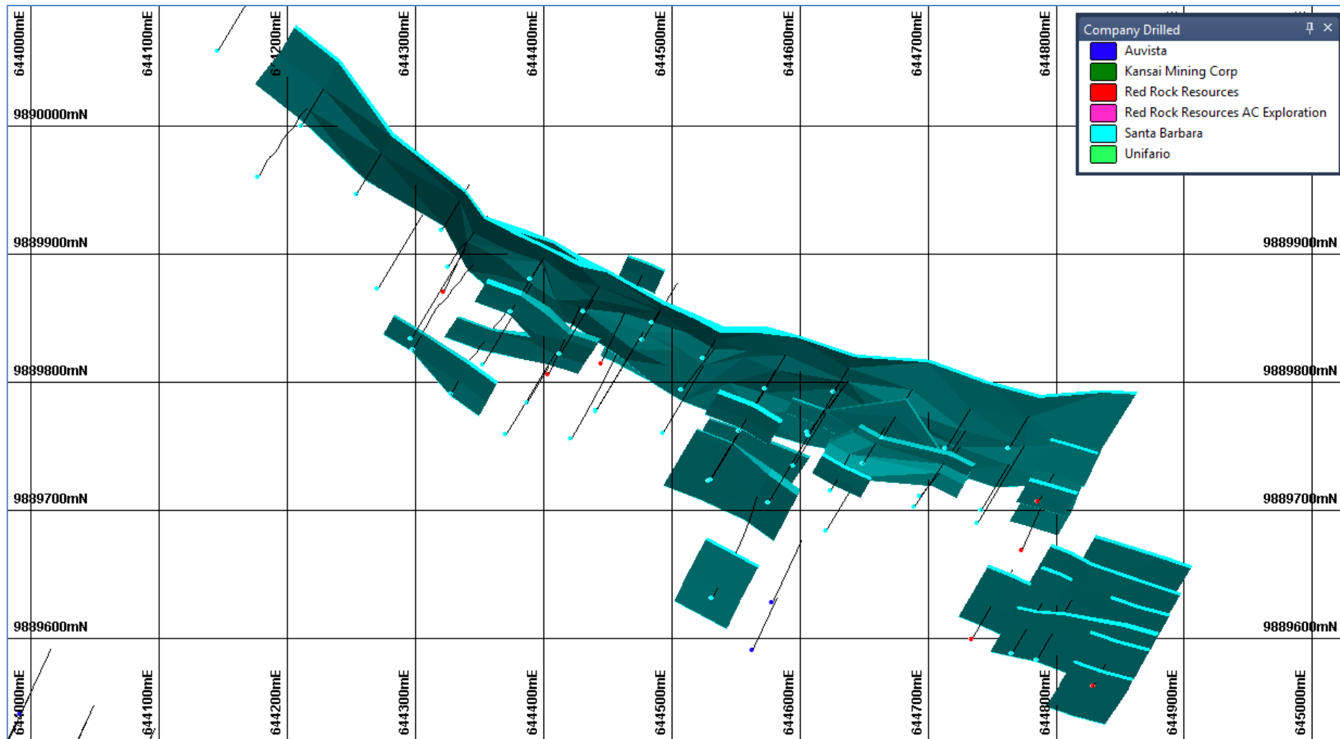
Figure 3 MK domain wireframes with drill holes coloured by company
