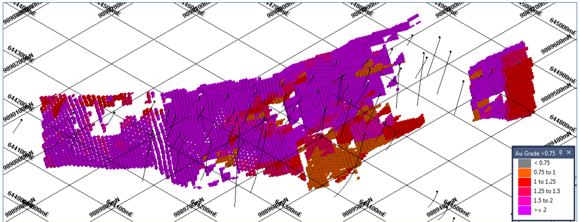
Figure 2 MRE block model for the MK prospect coloured by Au grade
