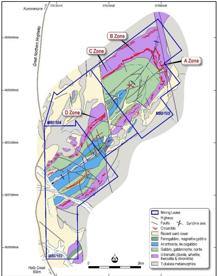
Figure One | Panton Geology Shown A, B, C and D Blocks
