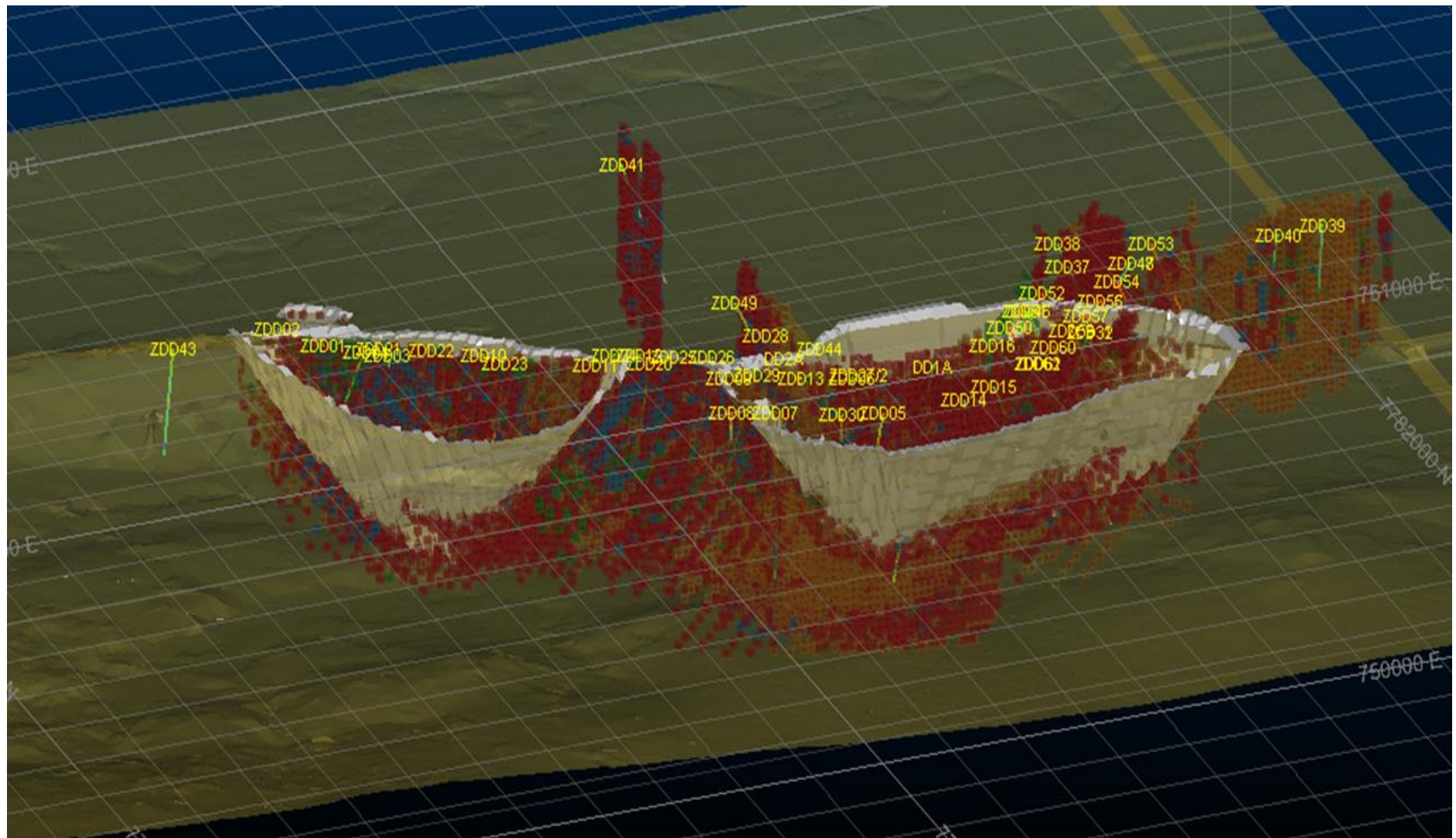
Image 2: Pit shell, step out zones and drill hole positioning
