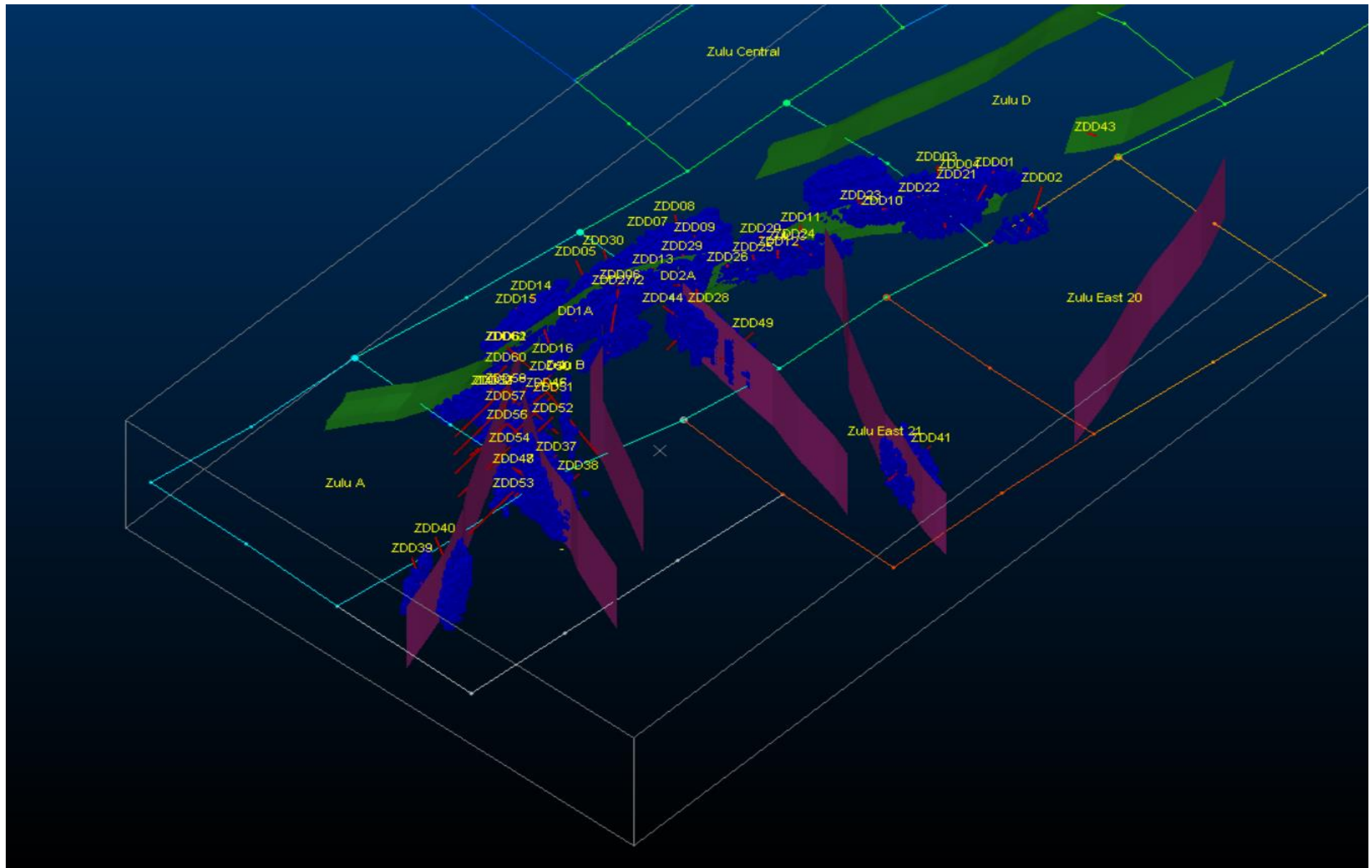
Image 4: Pit shell, step out zones and drill hole positioning
