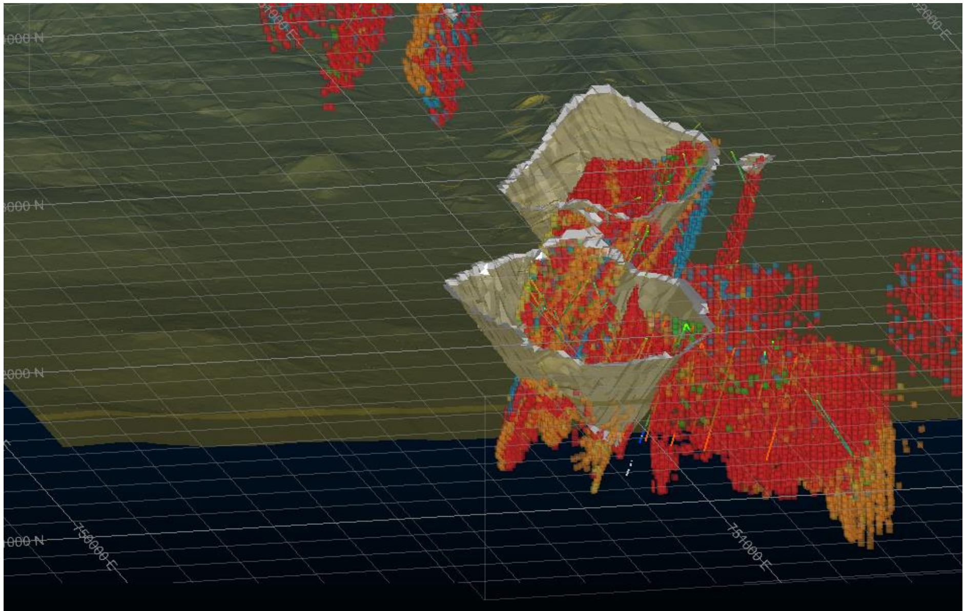
Image 3: Pit shell, step out zones and drill hole positioning
