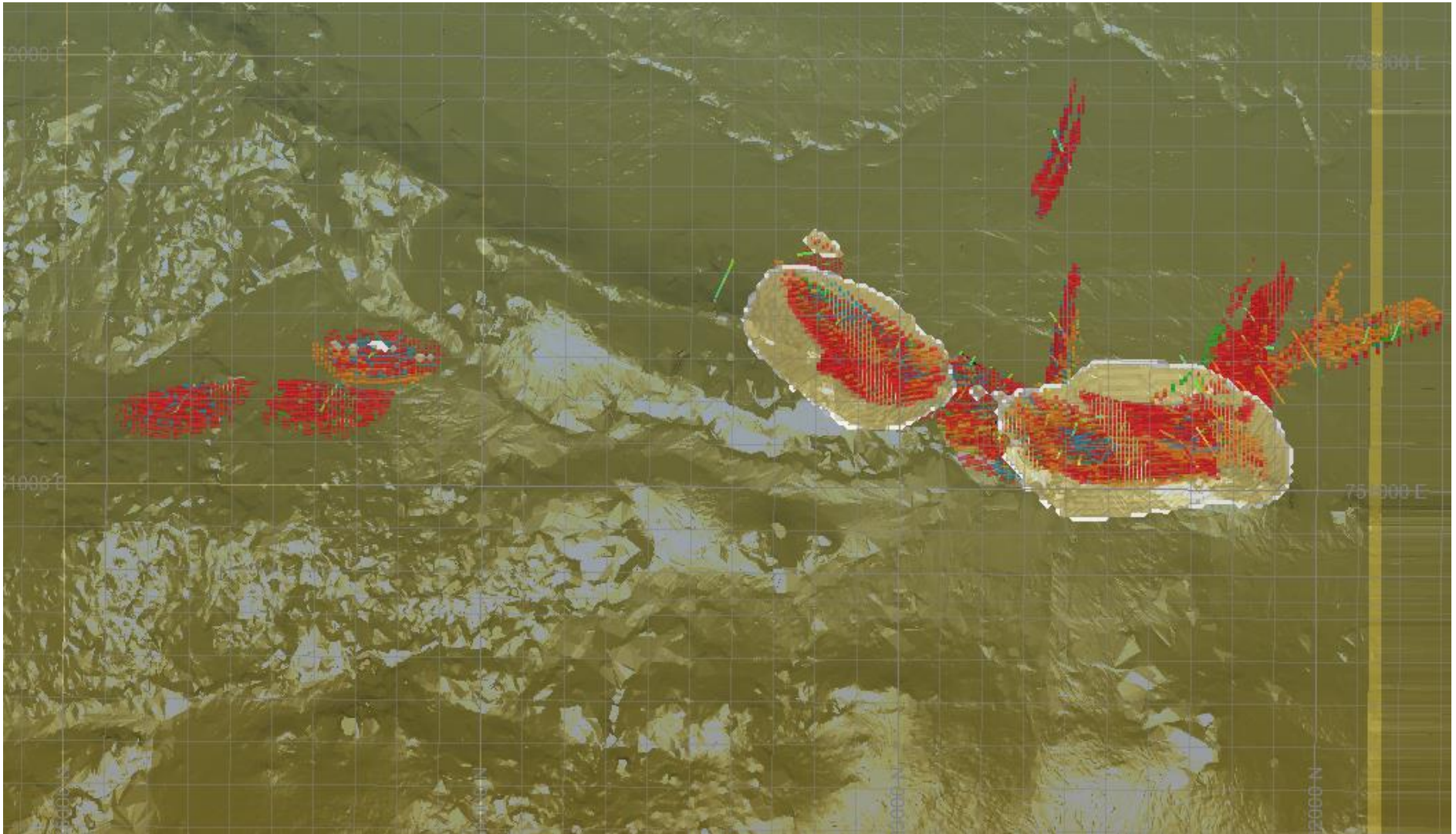
Image 1: Pit shell, step out zones and drill hole positioning
