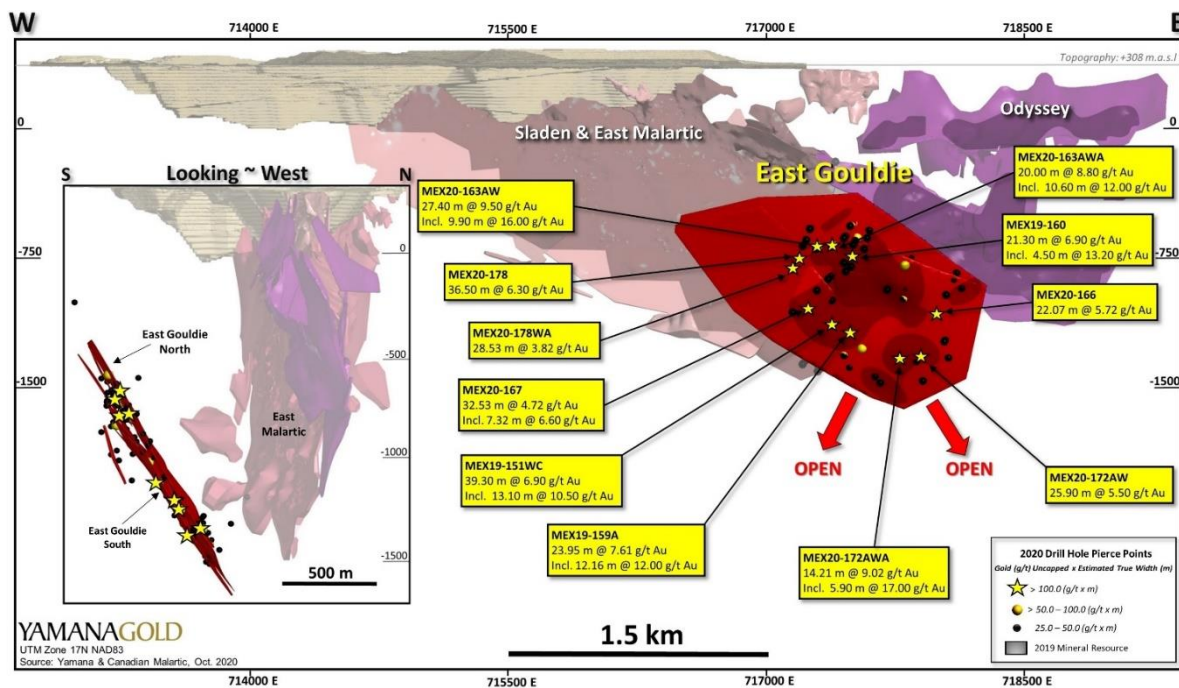
Figure 2: Canadian Malartic long section looking north, highlighting 2020 drilling results for the East Gouldie zone. Drilling intercepts presented include those greater than 25.0 gram*metres (Gold g/t (uncapped) multiplied by estimated true width in metres).
