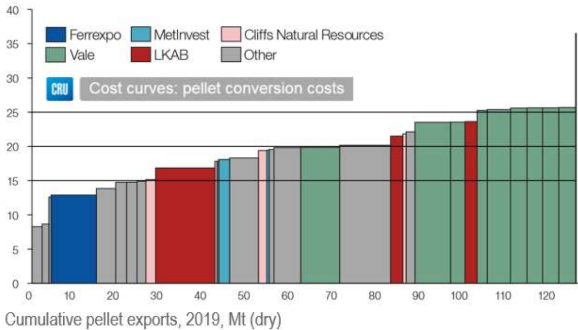
Graph 1: Pelletising conversion costs from pellet feed to pellet, 2019, ex-works, US$/dmt
