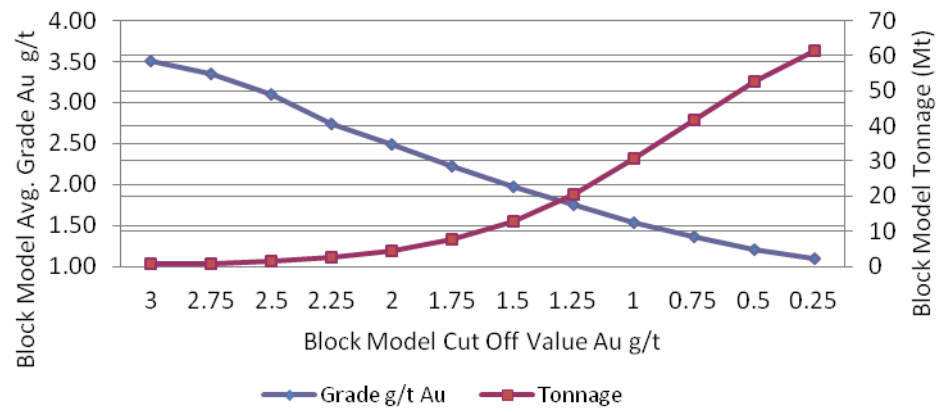
Grade Tonnage Curve for Tuzon Block Model All_20th Jan 2012
