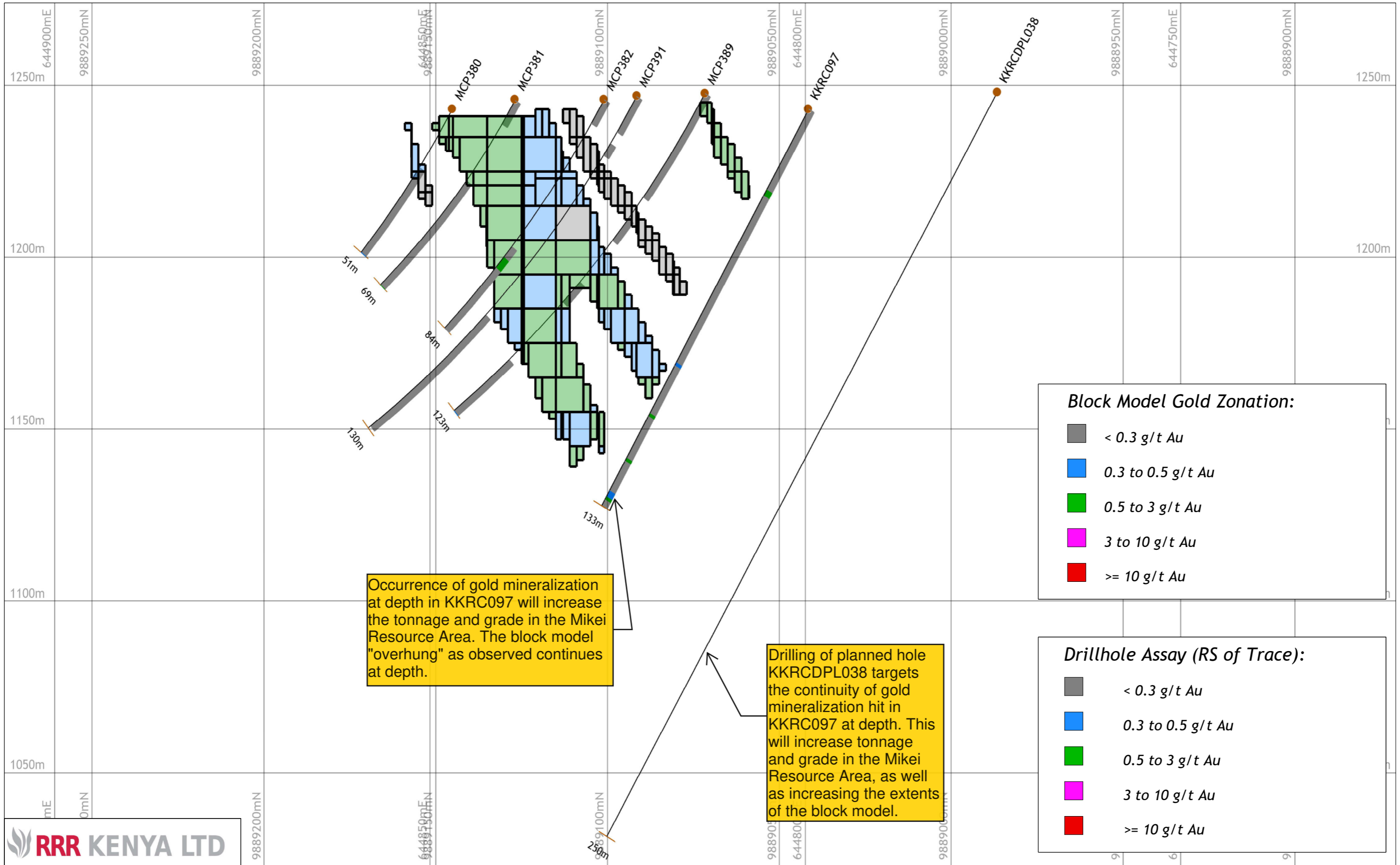
KKRC097: DRILLHOLE ASSAY VS BLOCK MODEL
