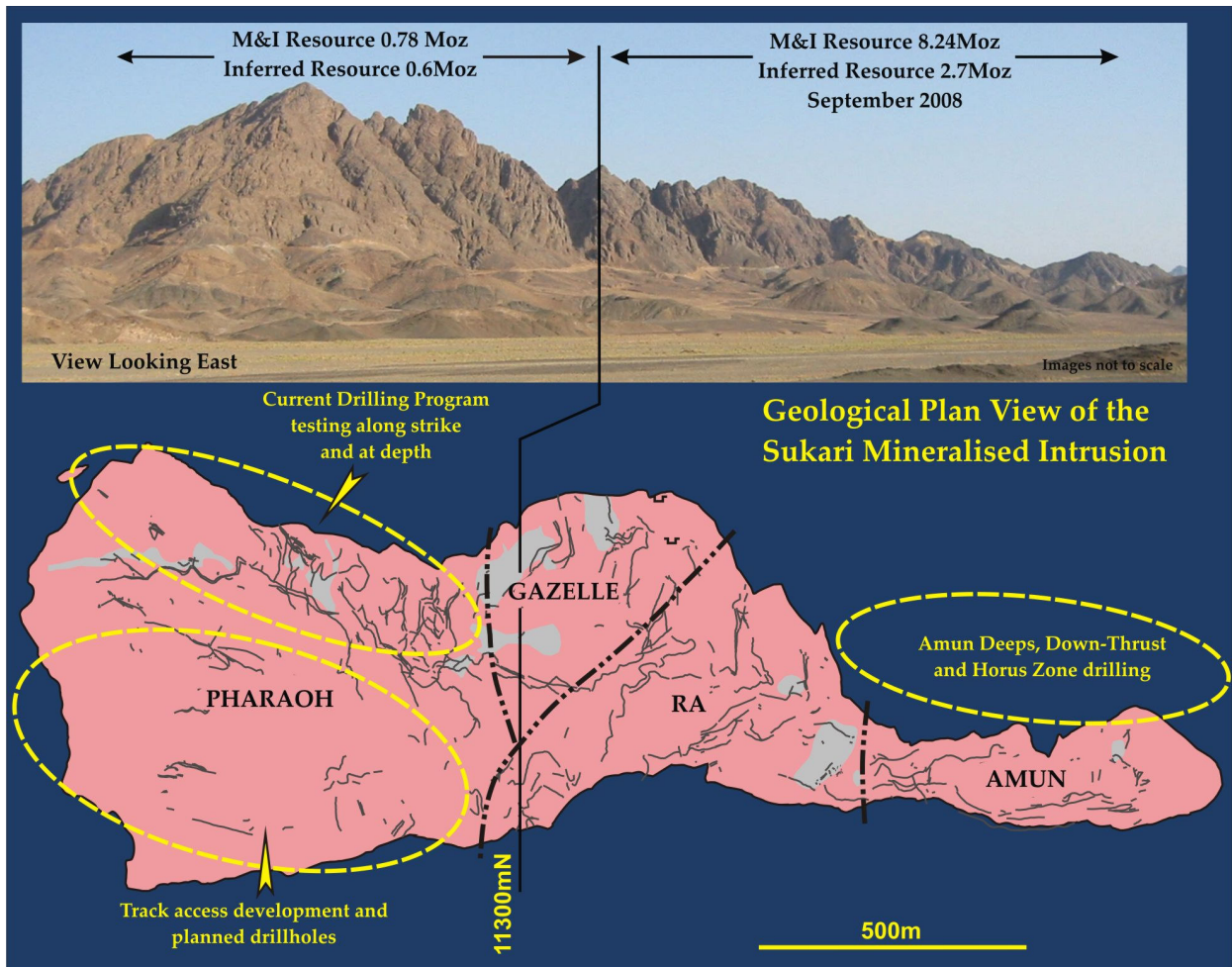
Figure 5 – Sukari outcrop and porphyry outline
