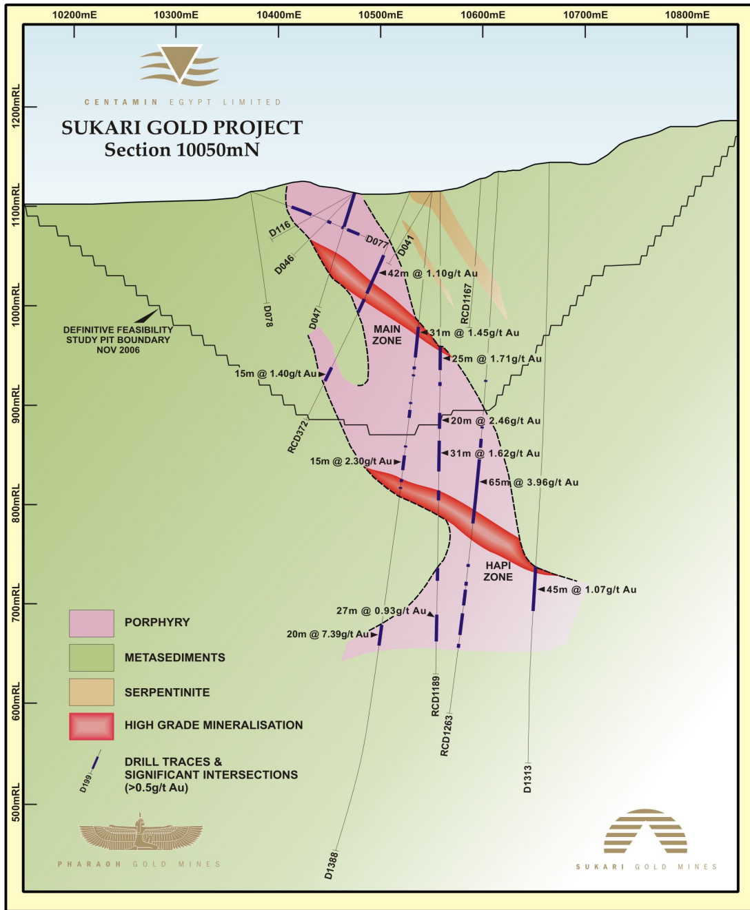
Figure 2 – 10050N – D1388 - high grade mineralisation in the downthrust zone at the base of Amun Deeps porphyry block
