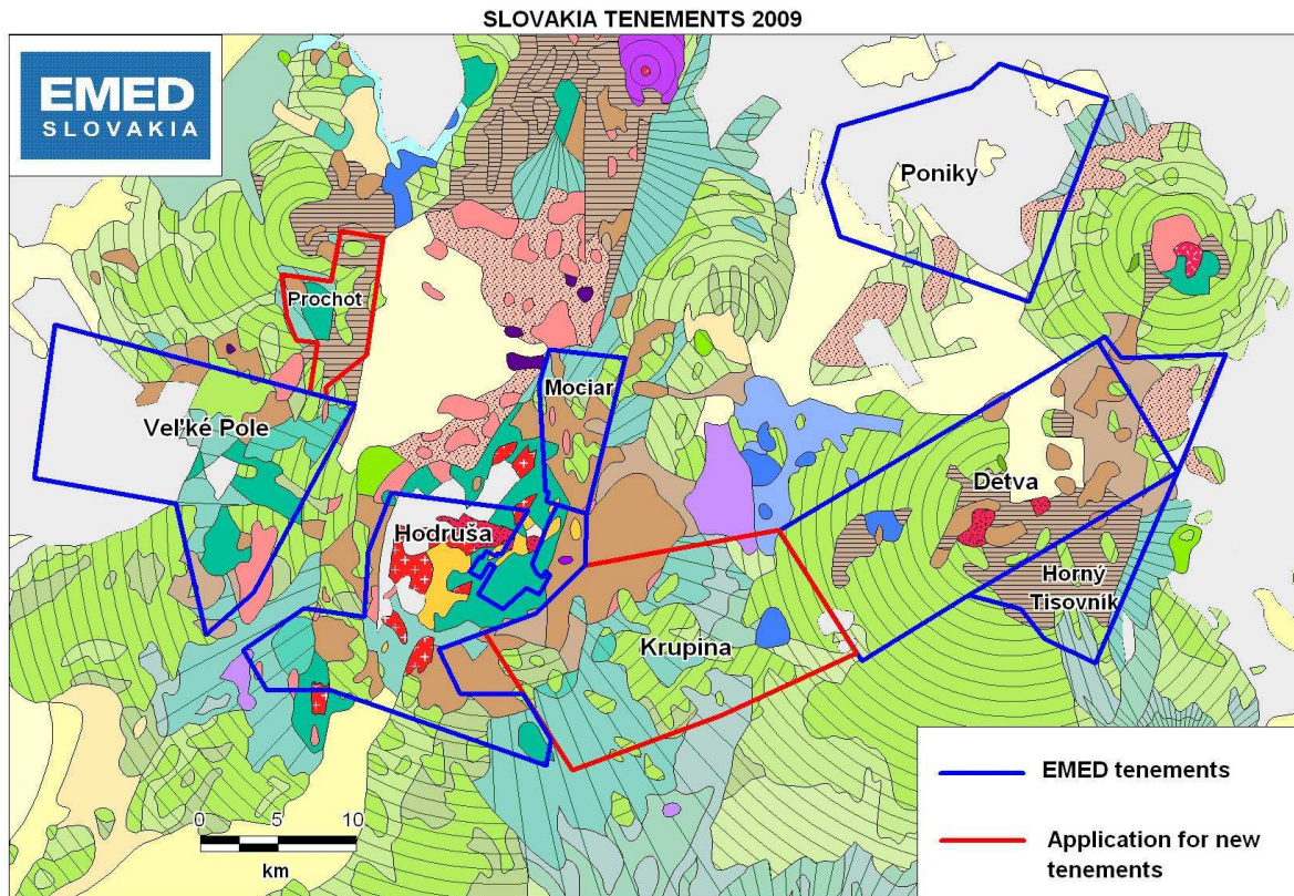
Diagram 2 - Slovakia Tenements 2009
