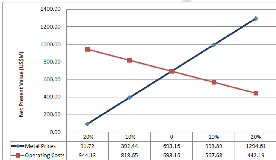
Graph showing metal price and operating cost sensitivity analysis for the RKEF process.
