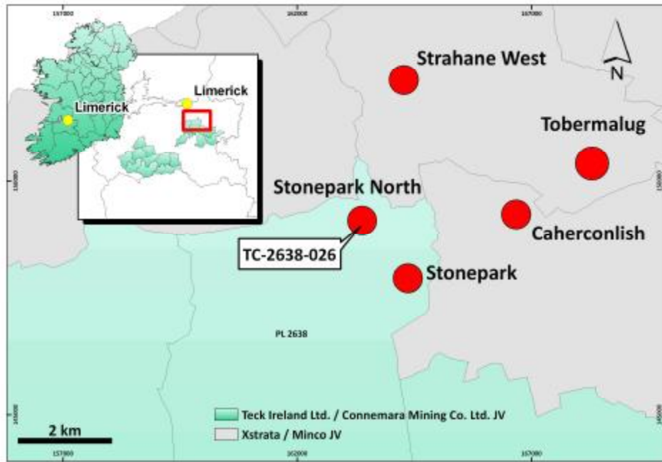
Figure 1: Zinc Discoveries in the Limerick Region
