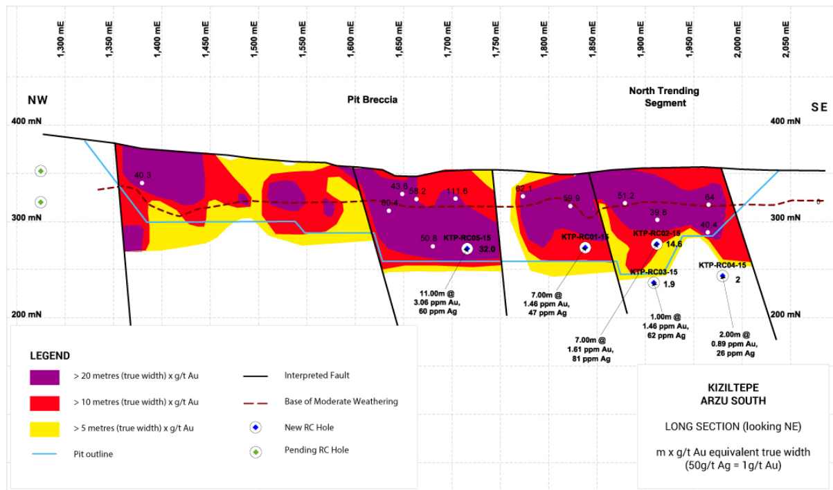
Figure 1: Long-section showing grade*thickness contours from drilling at the Arzu South vein, with new drilling results. The coloured regions represent true thickness gram x metre Gold equivalent intercepts. The gram x metre intercepts shown for the new holes also represent true thickness, though downhole mineralised intercepts are also labelled. True thickness intercepts >40m.g/t of Gold (pierce points) from previous drilling are also shown.
