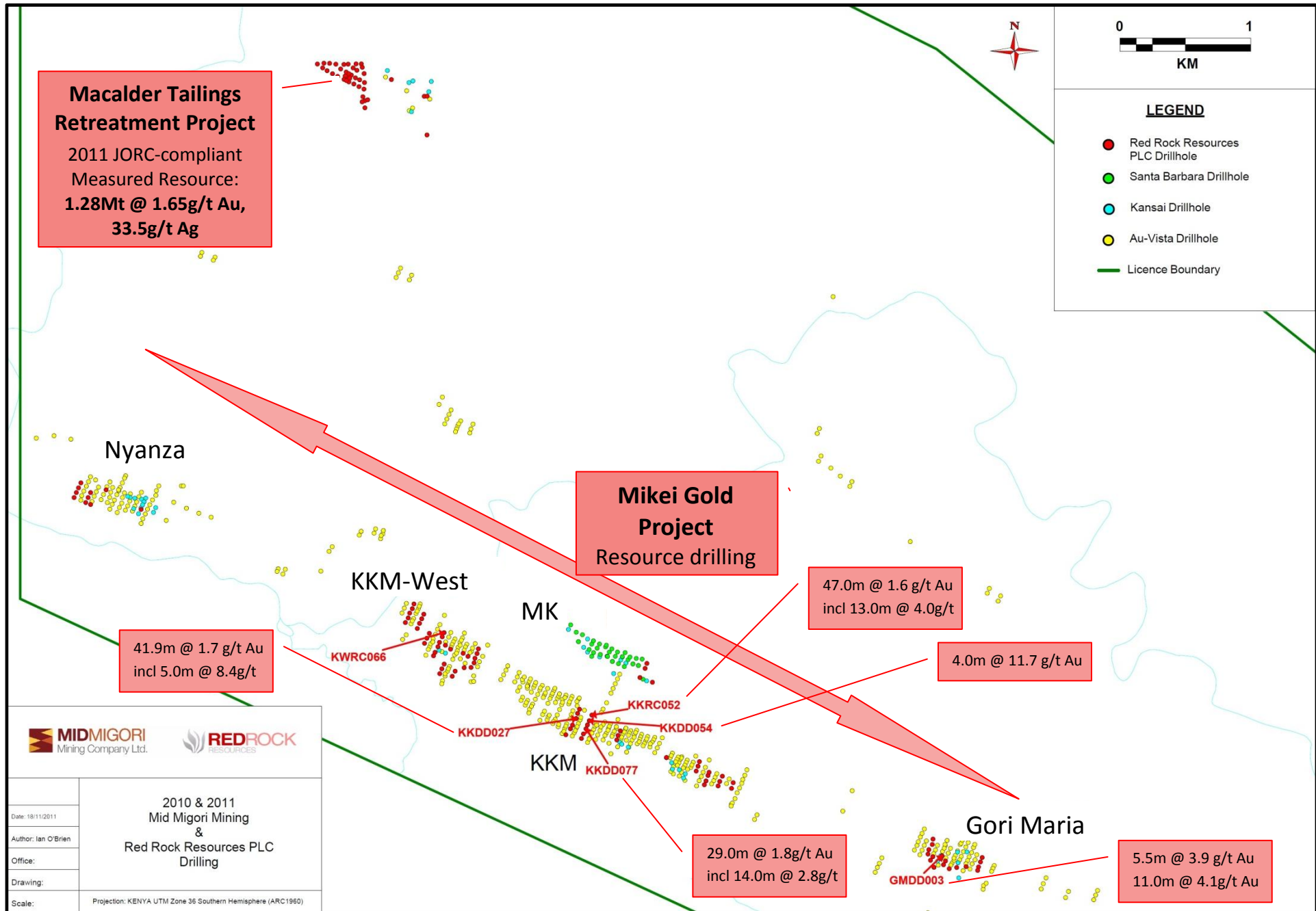
Figure 2: Mikei Gold Project Drilling Plan showing individual prospects subject to Mineral Resource Estimate updates, and recent key drilling results.
