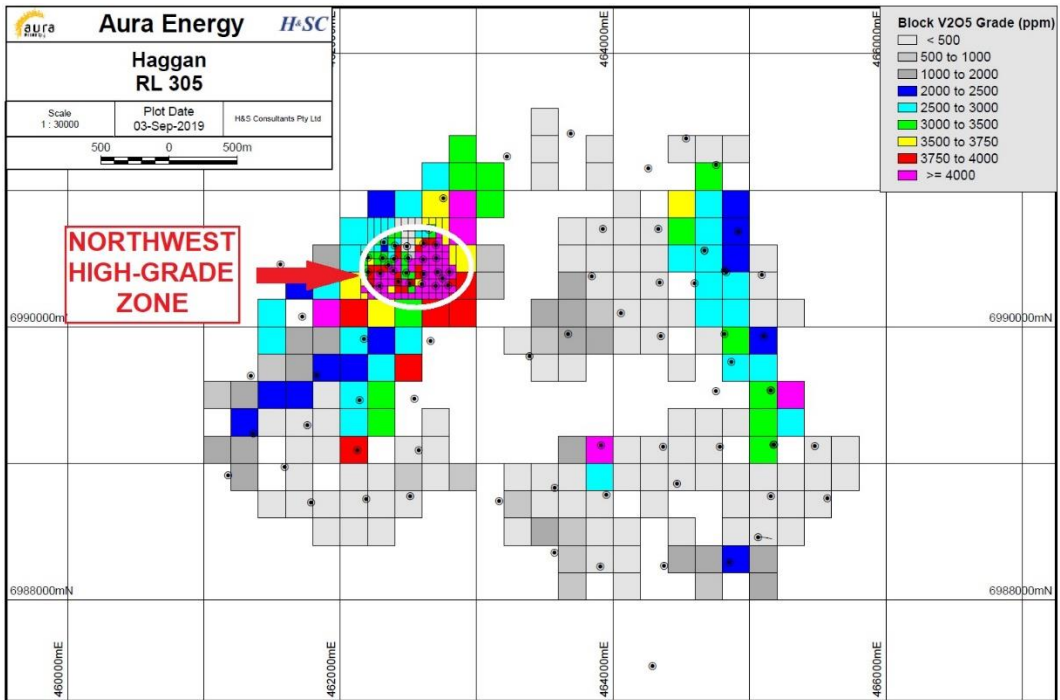
Figure 4: Horizontal section (plan view) of Häggån Resource at a depth of approximately 45 metres below surface
