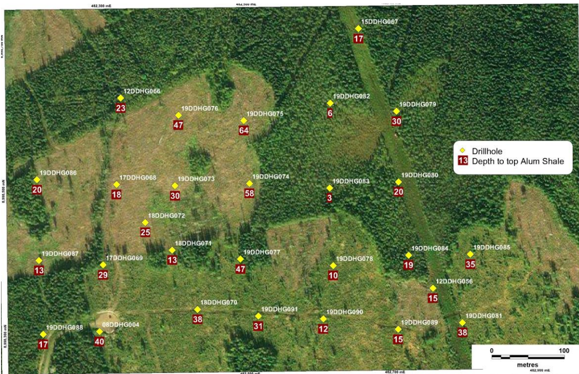
Figure 5. Plan of collars of drillholes on which the Indicated Resource is based.
