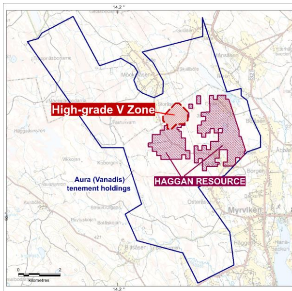
Figure 2: Situation of the High-Grade vanadium zone within the Haggan Resource. The mineral tenements are held 100% by Aura's 100% owned Swedish subsidiary Vanadis Battery Metals AB.
