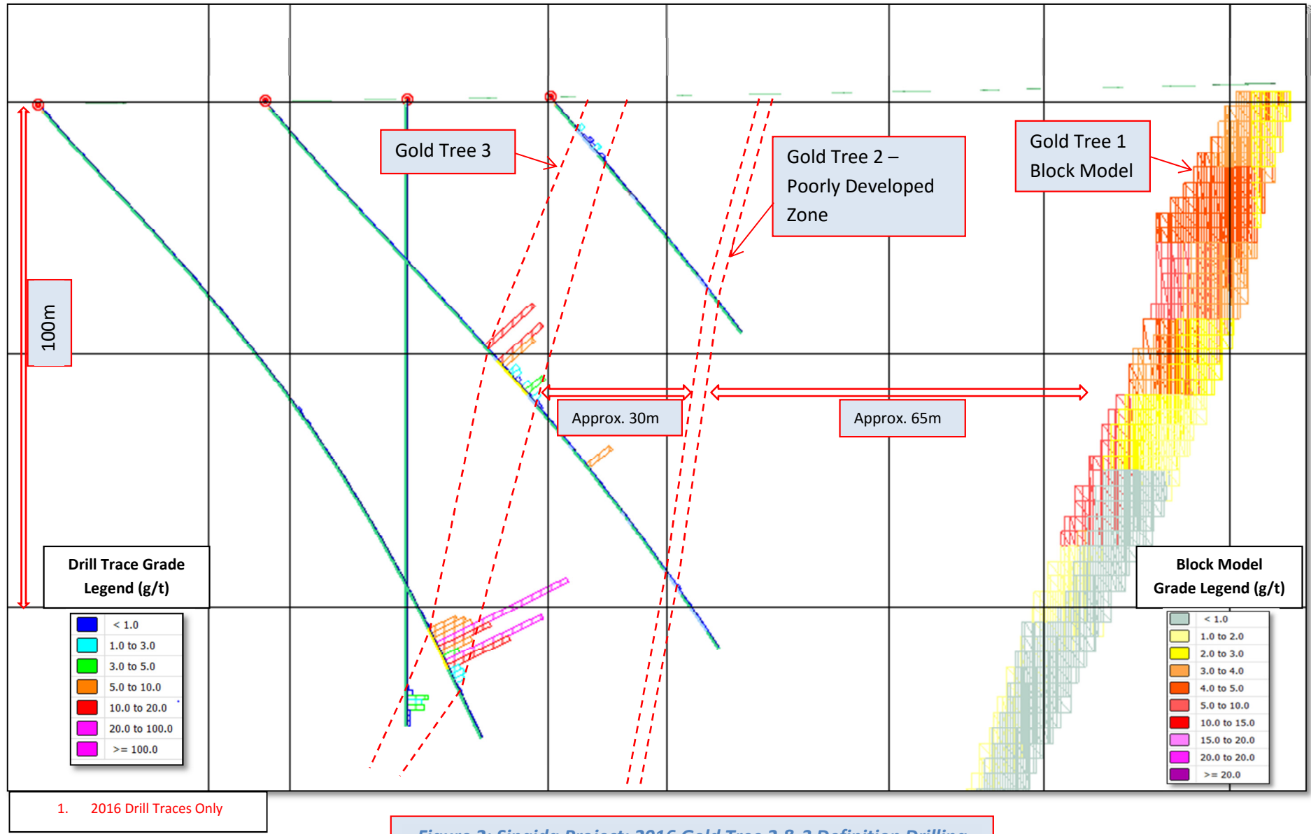
Figure 2: Singida Project: 2016 Gold Tree 2 & 3 Definition Drilling Drilled Section looking Northwest – Section 1
