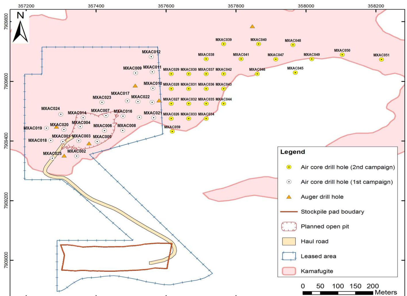
Figure 02 – Plan of initial civil and infrastructure works and open pit area for trial mining alongside location of previous and new resource drill holes.
