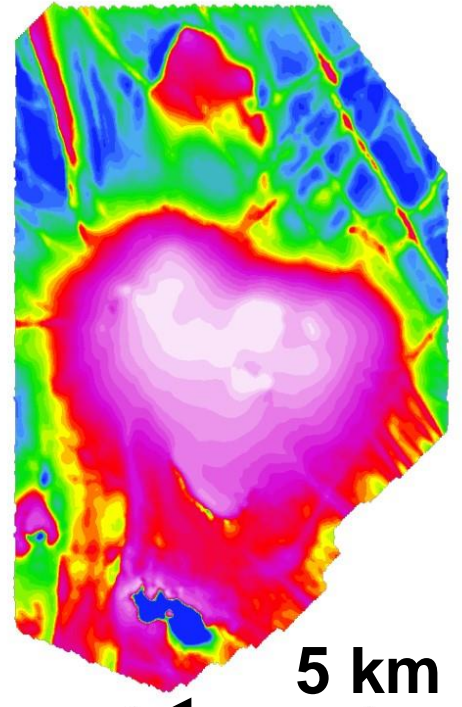
Rockfire's helicopter magnetics RTP (Reduced to Pole)
