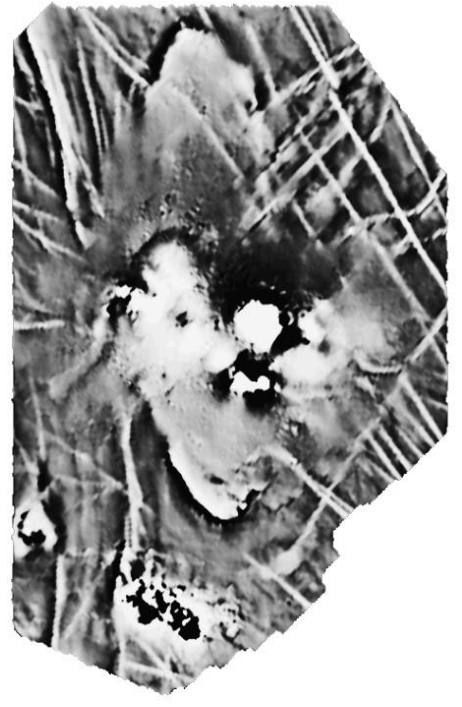
Rockfire's helicopter magnetics 1VD (1st Vertical Derivative)
