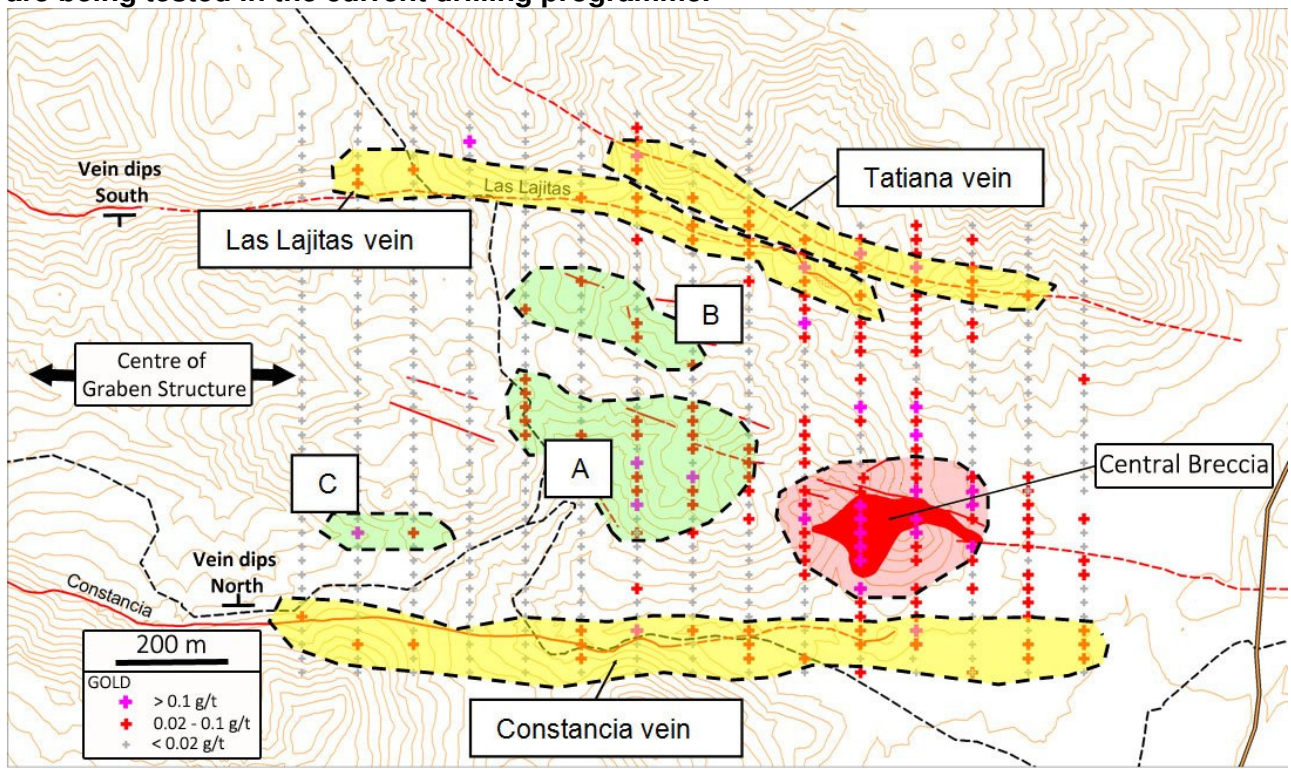
Figure 2. Location of Central Breccia and soil anomalies. The stronger anomalies A and B are being tested in the current drilling programme.
