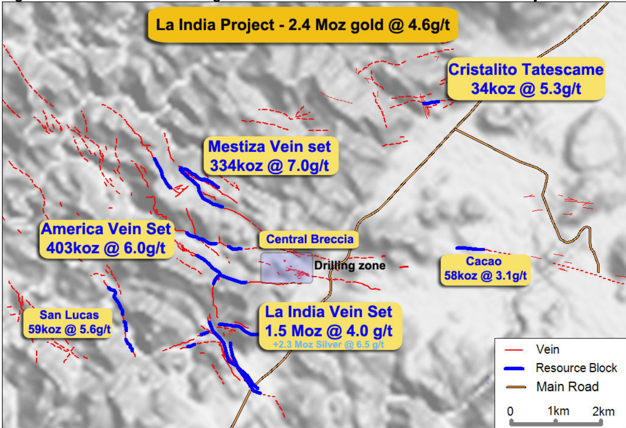
Figure 3. Location of the Drilling on the Central Breccia within the La India Project area.
