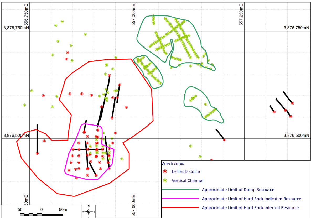
Figure 1, overview map of exploration drilling and channel sampling, with approximate surface expression of resources.
