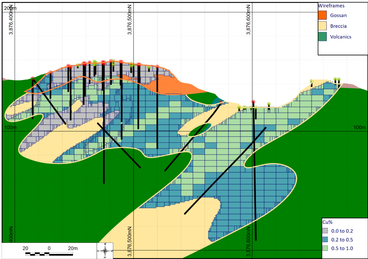
Figure 2, example cross section of hard rock Cu resource.
