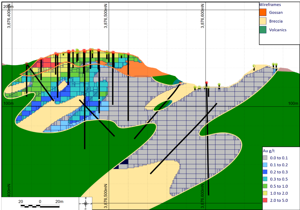
Figure 3, example cross section of hard rock Au resource.
