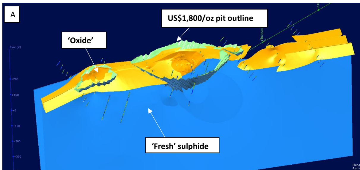
Figure 2A to C: Series of images showing the Faré South wireframe models relative to the US$1,800/oz Resource pit shell. Pit outline is in green, blue shapes represent 'fresh' sulphide mineralisation, orange shapes represent 'oxide' mineralisation.
