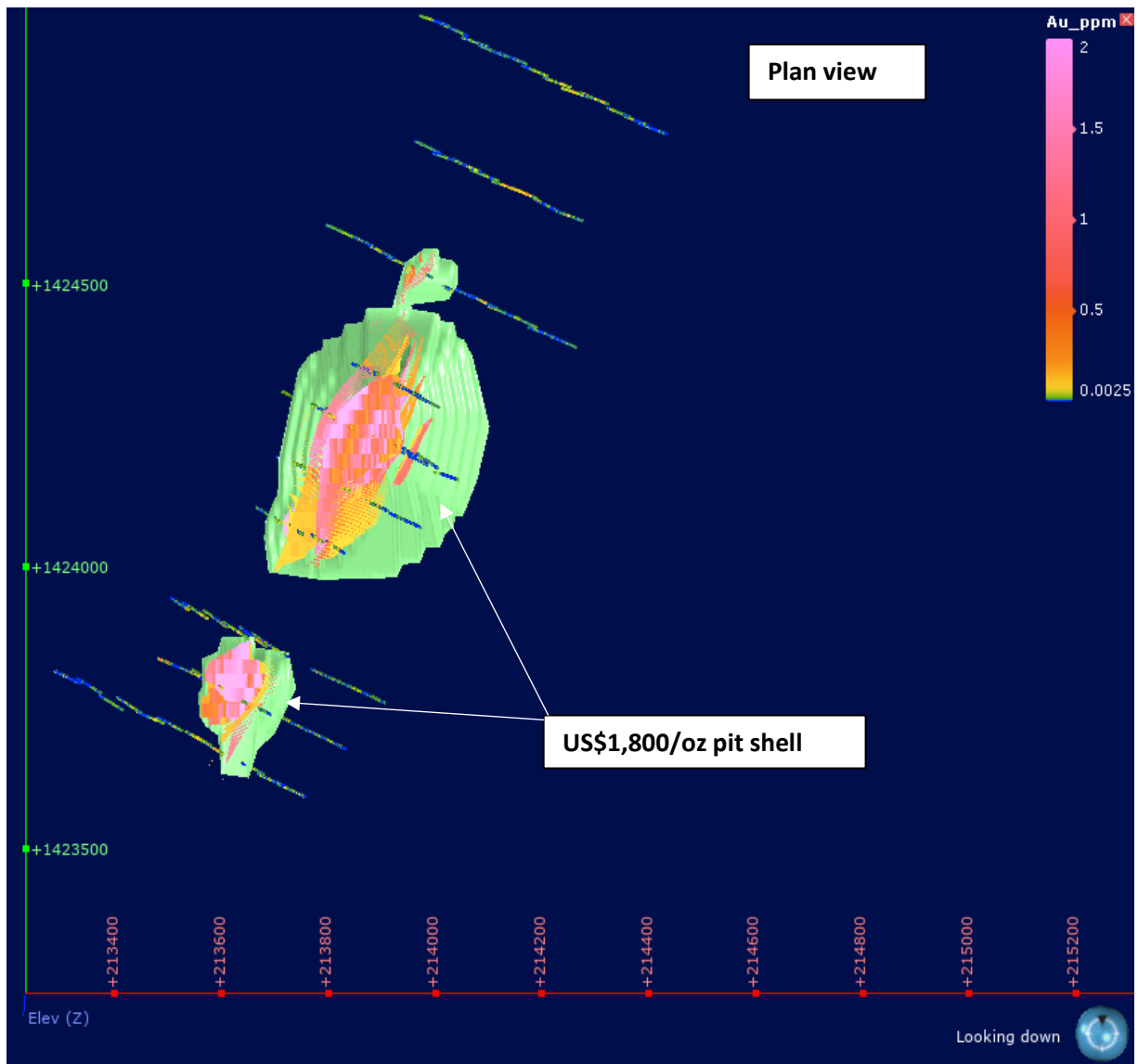
Figure 1: Plan view of the Faré South block model, constrained to show blocks above a 0.3 g/t cut-off within a US$1,800/oz Resource pit shell. Downhole colouration also corresponds to Au grades shown in legend.
