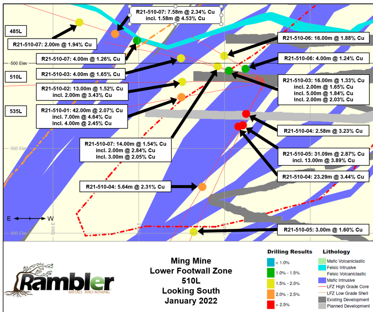
Figure 2: 510L LP East Zone drilling intersections
