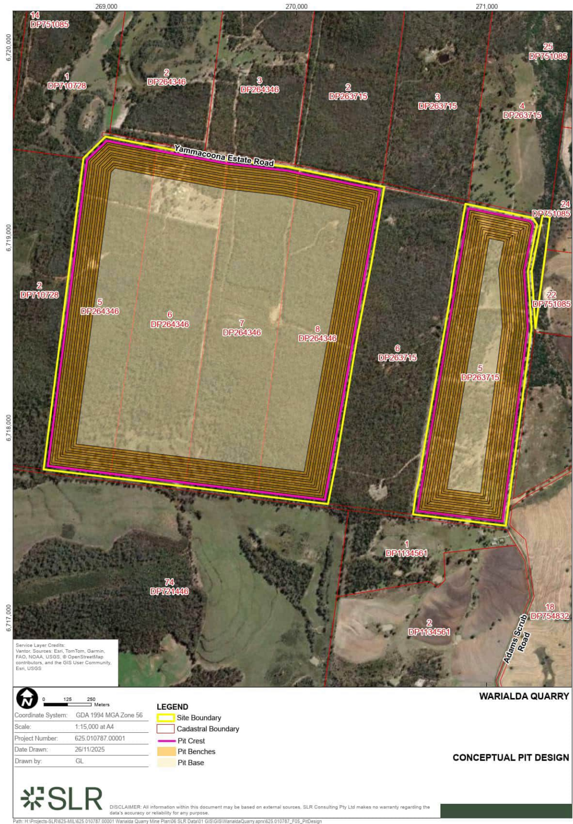
Figure 7 - Concept Pit Design
