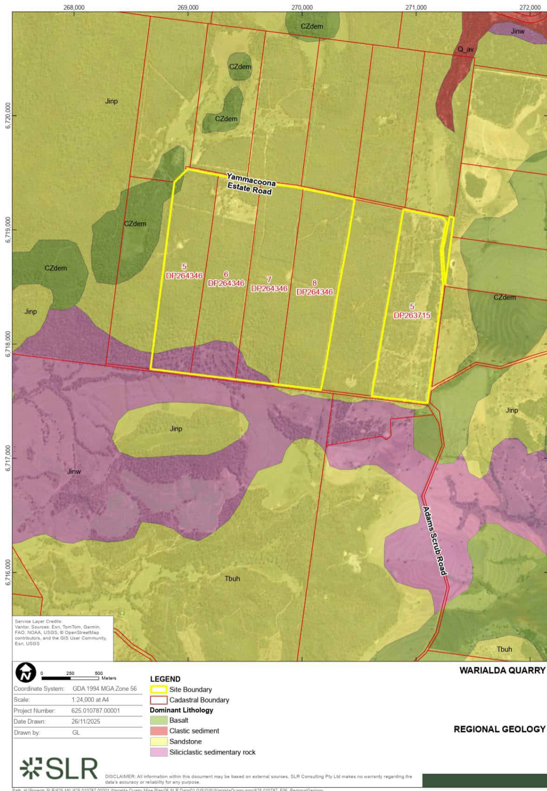
Figure 3 - Regional Geology
