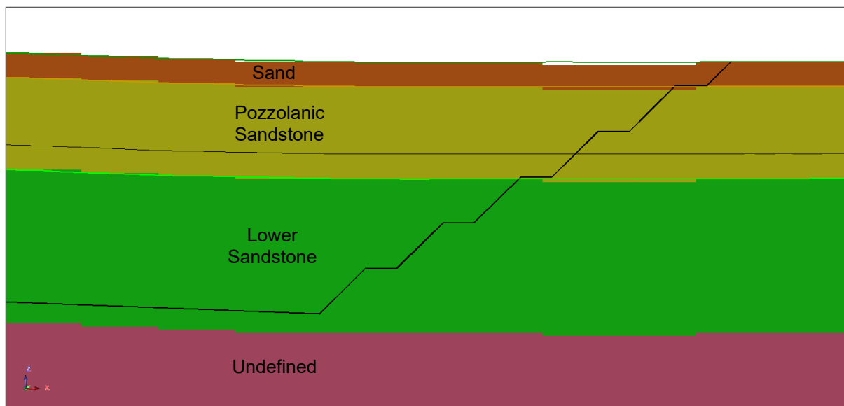
Figure 5 - Geological Profile
