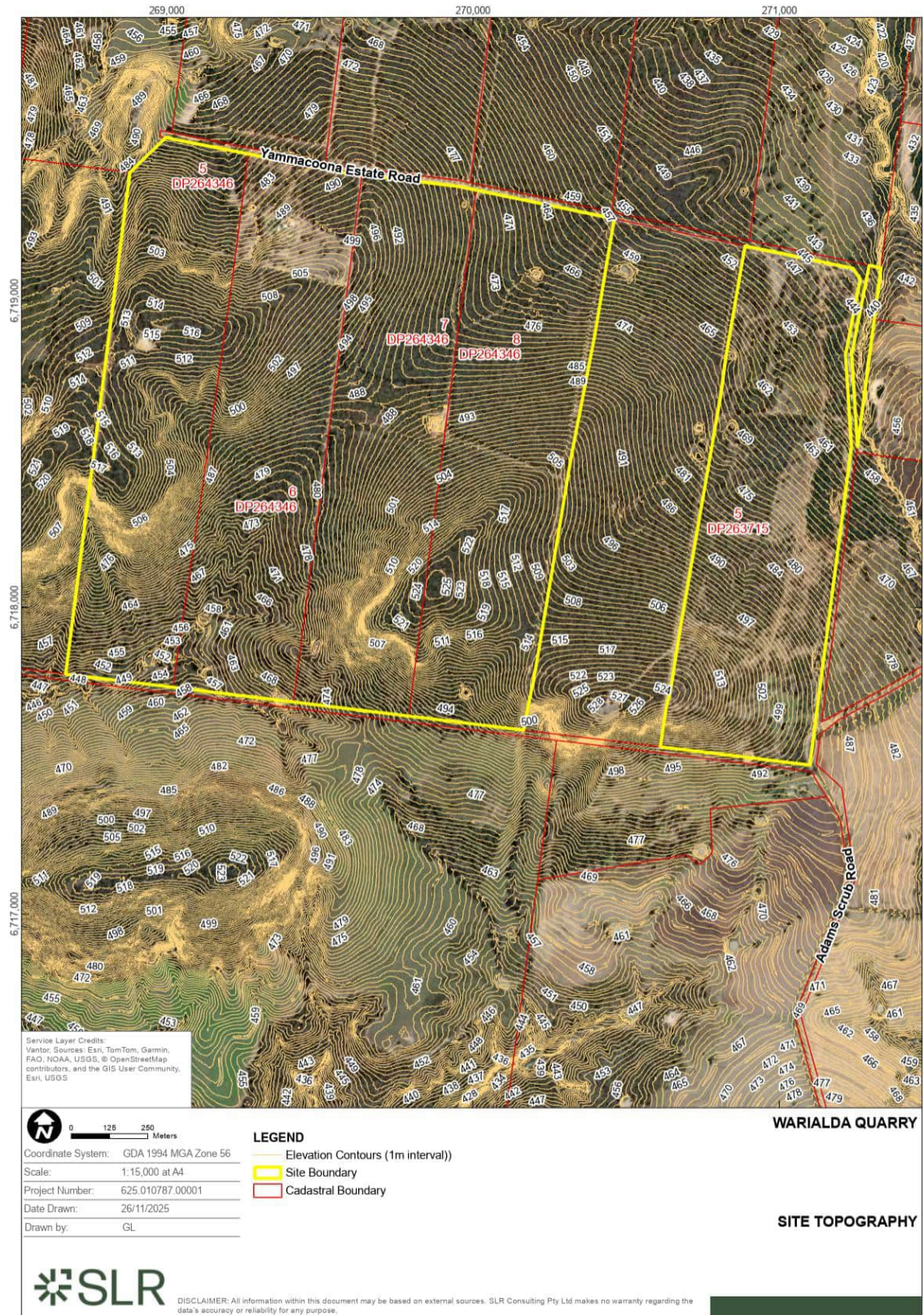
Figure 6 - Topographic Contours
