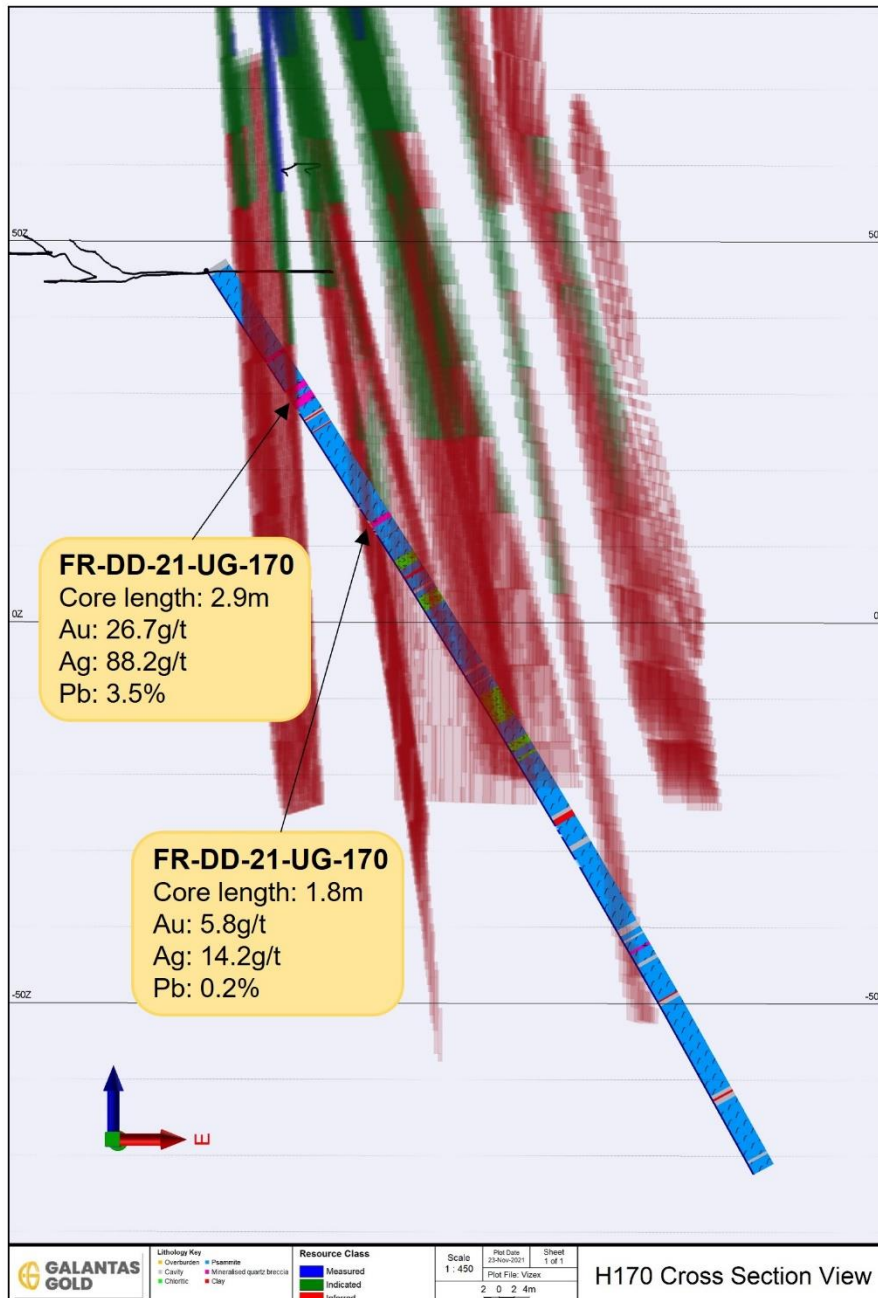
Figure 3: Cross-section showing results for recent hole FR-DD-21-UG-170.
