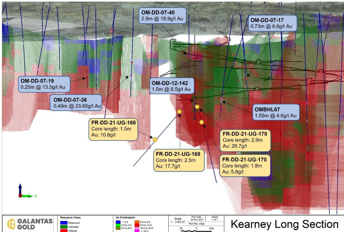
Figure 1: Kearney long-section view showing part of the resource model, the underground development, some key vein intersections and the first two holes FR-DD-21-UG-168 and 170.
