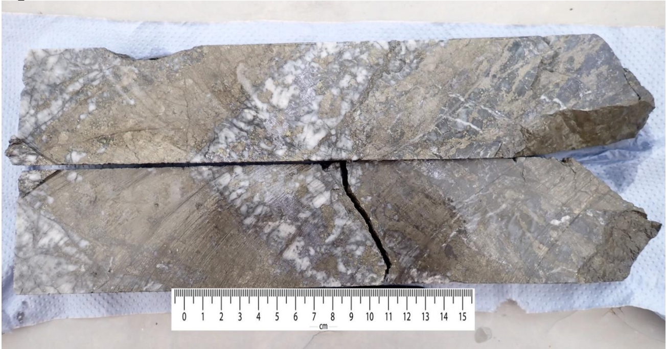
Figure 2: Drill core from hole FR-DD-21-UG-170.
