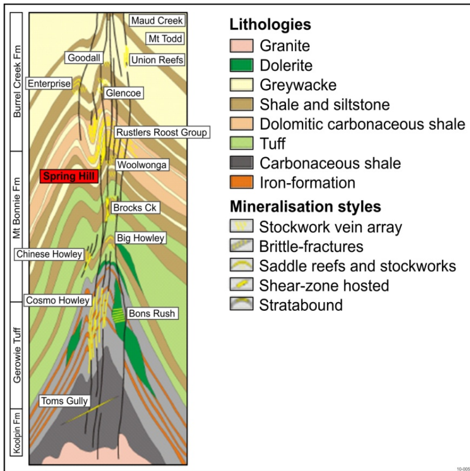
Figure 7: Structural and stratigraphic setting and styles of gold mineralisation in the Pine Creek Inlier (After N.T. Geological Survey)
