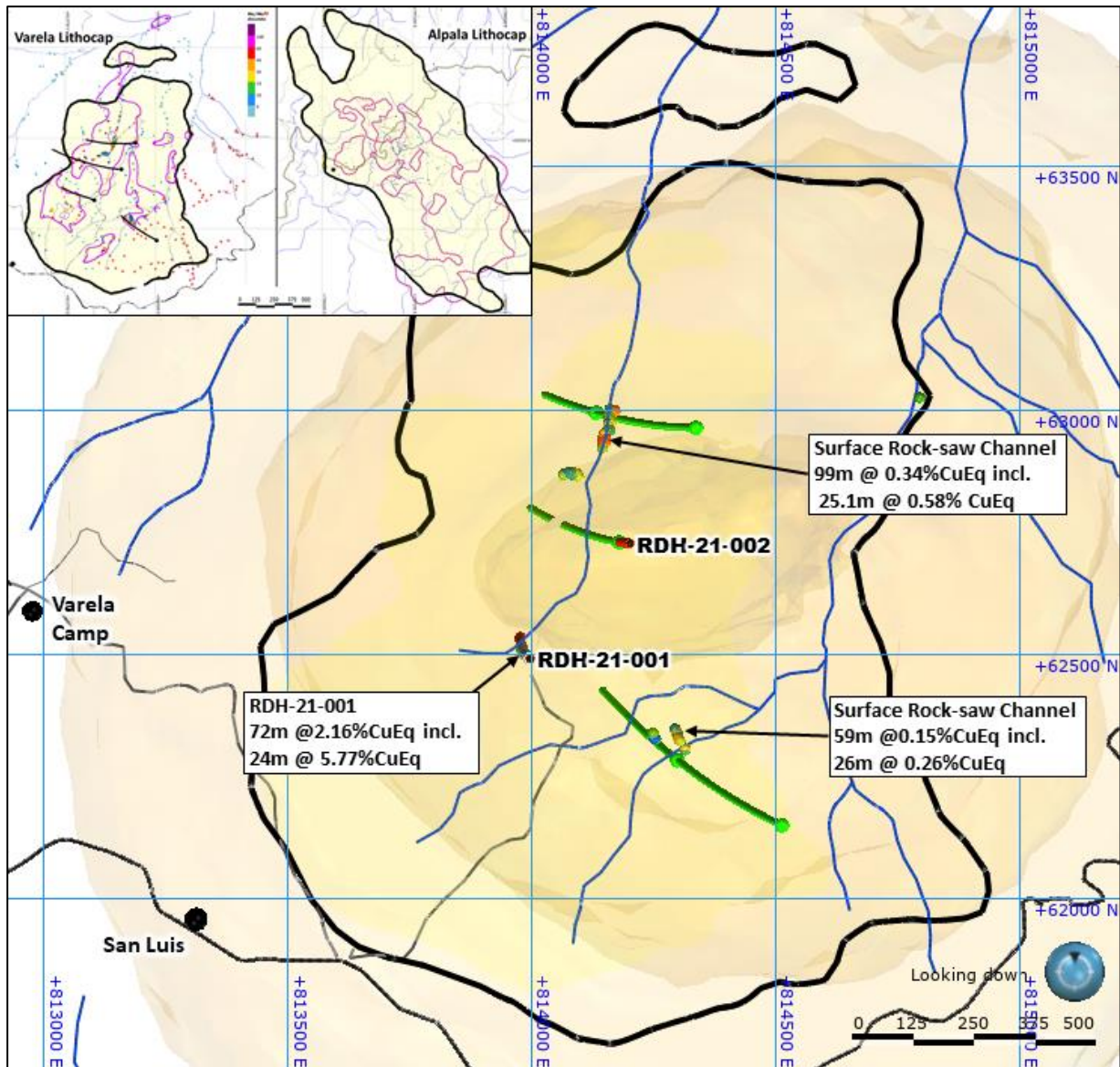
Figure 3: Plan view of Varella target, showing SolGold’s Varella Camp, the mapped lithocap area (thick black outline), over Halley & Cohen 3D geochemical targets (yellow shading). Assay results from Hole 1 and surface outcrops are shown, and current drill hole path of RDH-21-002 is shown in red, planned drill holes are shown in green. The overall size of the Varella Mo/Mn anomaly exceeds 1,200m x 800m, which is of similar size to the zone of anomalous Mo/Mn at Alpala (see inset comparison in the upper left-hand side of the figure).
