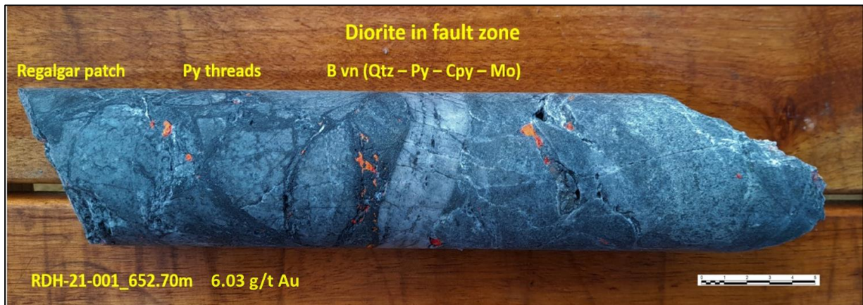
Figure 5: Portion of mineralised core within a 2-m interval that returned 6.03 g/t Au from a chlorite-sericite- and phyllic-altered fault zone in diorite with porphyry-style B-type quartz veins that contain pyrite (Py), chalcopyrite (Cpy) and molybdenite (Mo). Realgar (orange As-sulphide) occurs along late-stage fractures.
