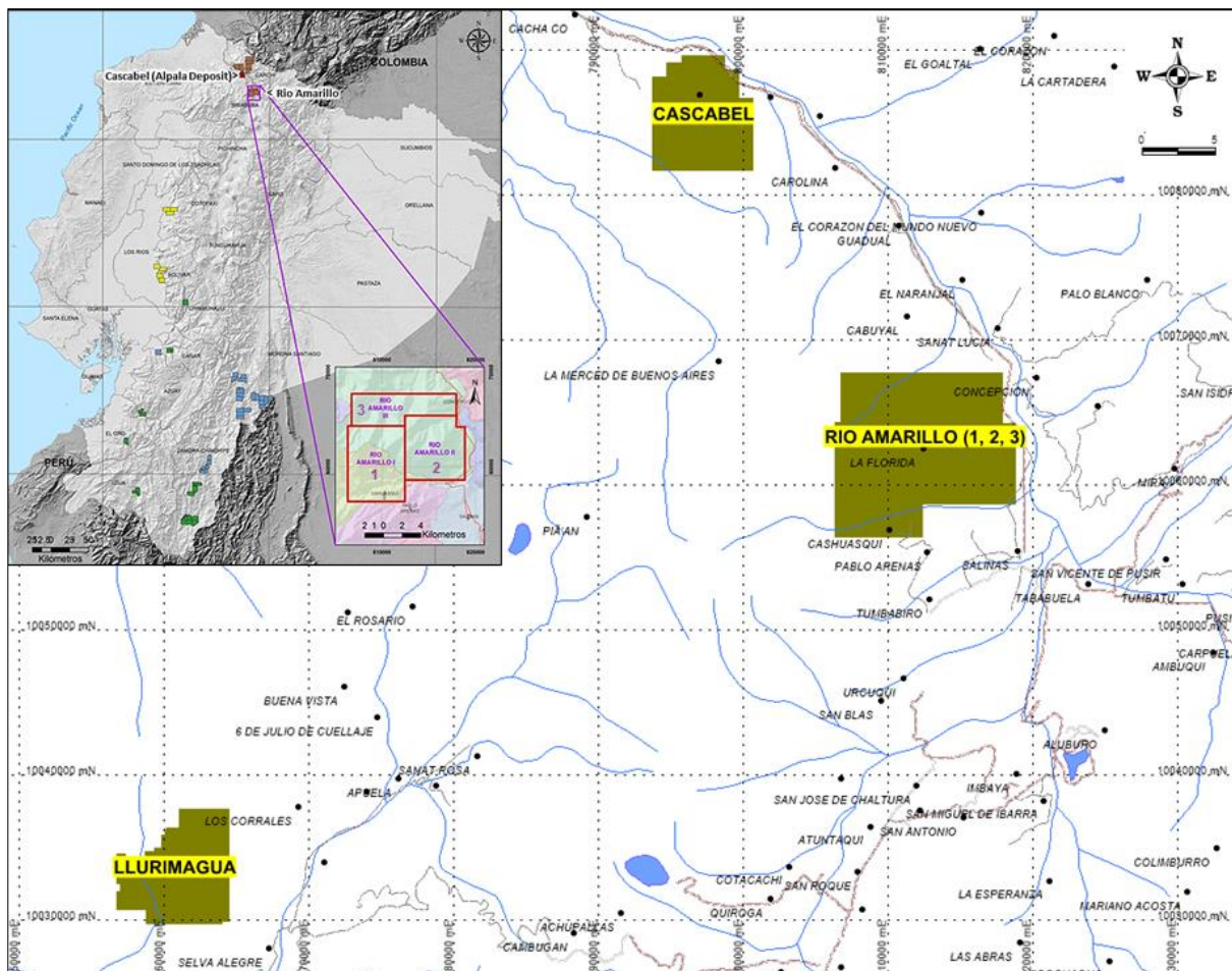
Figure 1: Location plan showing the Rio Amarillo project location in relation to the Alpala (SolGold) and the Llurimagua (ENAMI-Codelco) deposits. The Rio Amarillo project holds similar infrastructure advantages to the Alpala Project.
