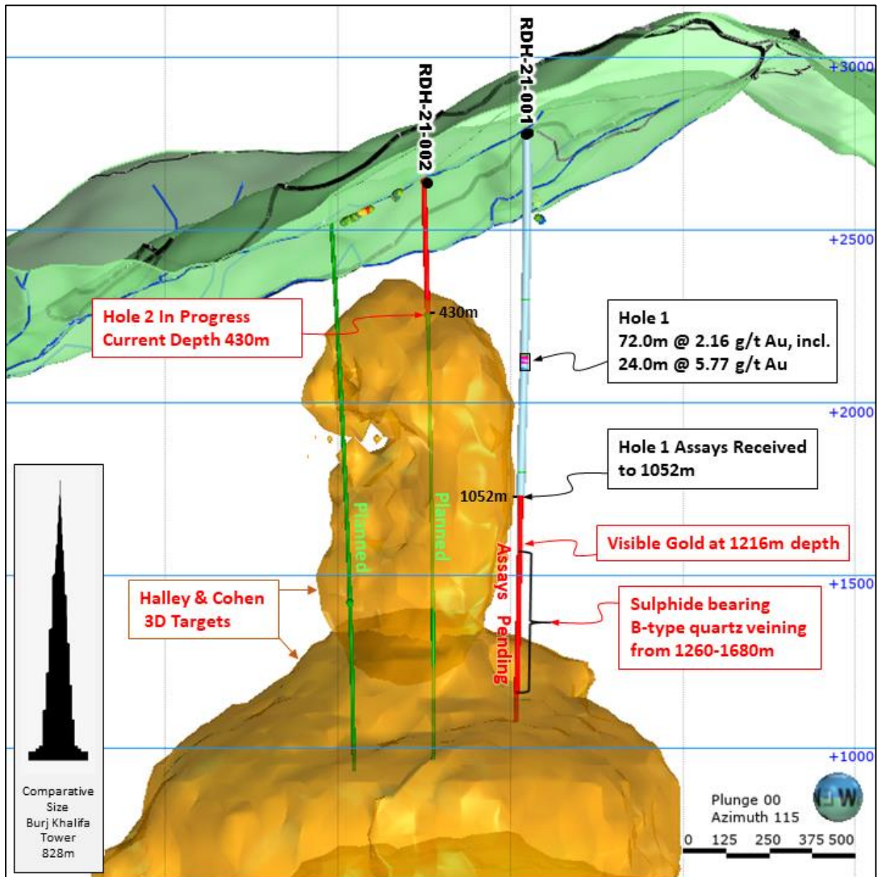
Figure 4: Sectional view looking east-southeast towards an azimuth of 115°, showing Halley & Cohen 3D geochemical targets (yellow), assay results from Hole 1, current drill hole path of RDH-21-002 (red), and planned drill holes (green). 3D geochemical modelling indicates a vertically extensive target zone seated directly beneath the Varela lithocap area. The model indicates potential for a porphyry copper deposit at depth, based on the comparison of geochemical zoning at Varela to the Yerington porphyry deposit in Nevada (Cohen, 2011; and Halley et al., 2015).
