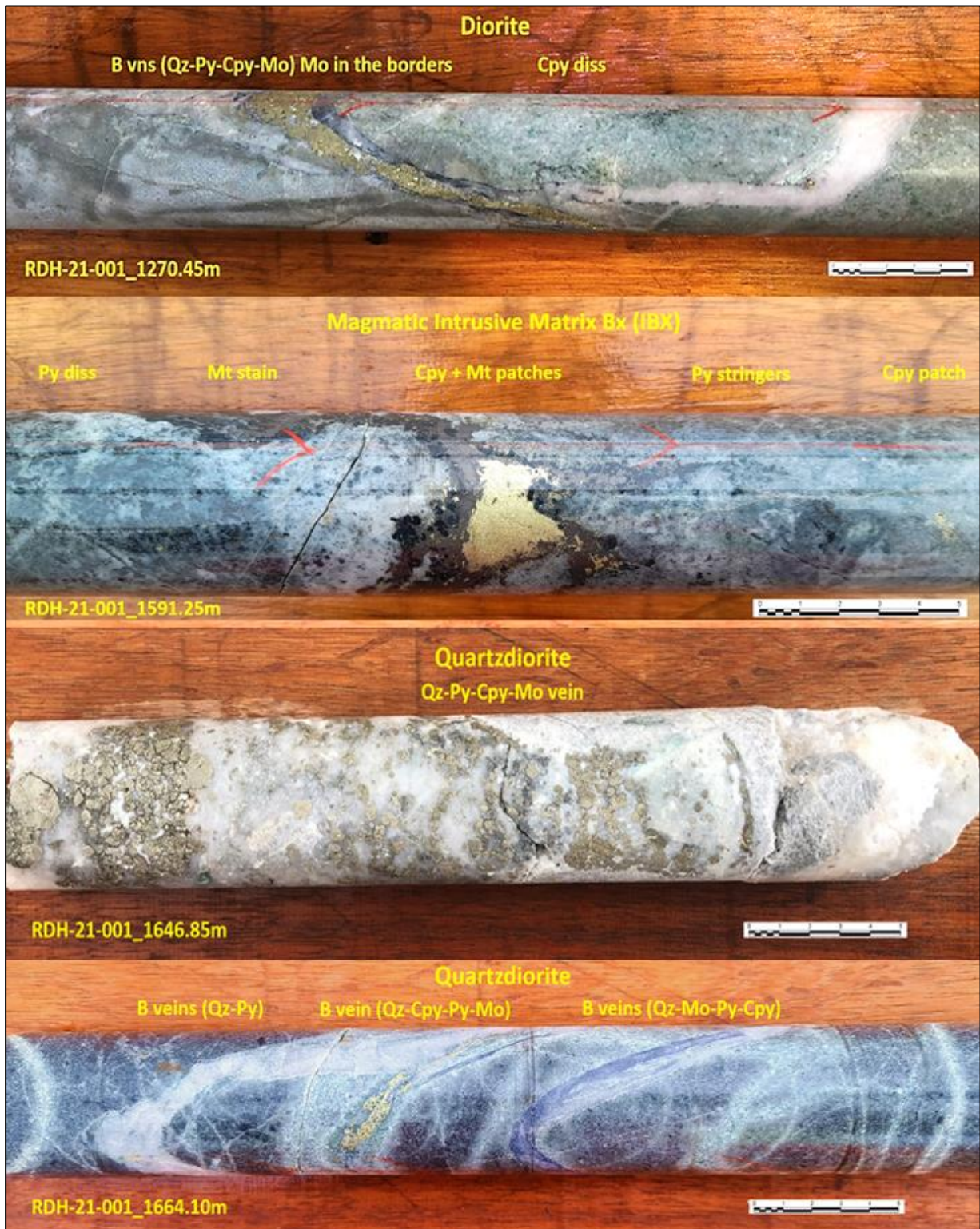
Figure 7: Core photos taken from various depths showing B type quartz veins with sulphide mineralisation (chalcopyrite-pyrite-molybdenite) associated with early biotite-potassic alteration overprinted by chlorite-sericite-clay alteration of diorite, quartz diorite and magmatic intrusive breccia.
