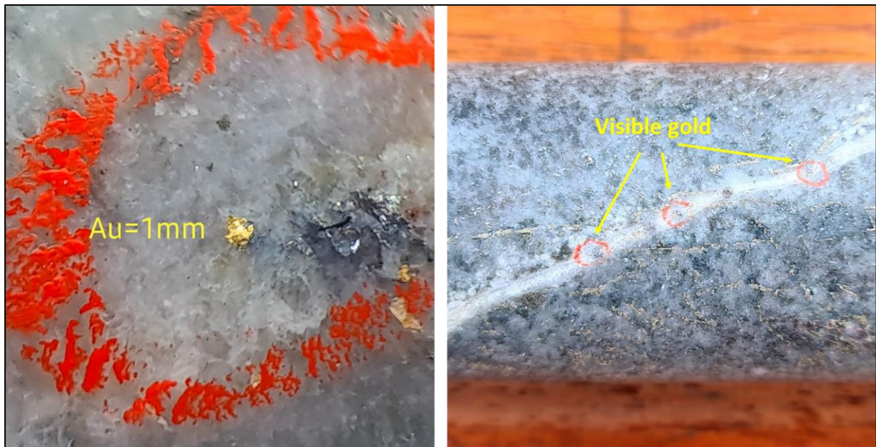
Figure 6: Sections of drill-core at 1,216.0m down-hole that contain multiple occurrences of visible gold, up to 1mm in mean-diameter, within a quartz-carbonate-gold-molybdenite vein hosted in chlorite-sericite-altered diorite.
