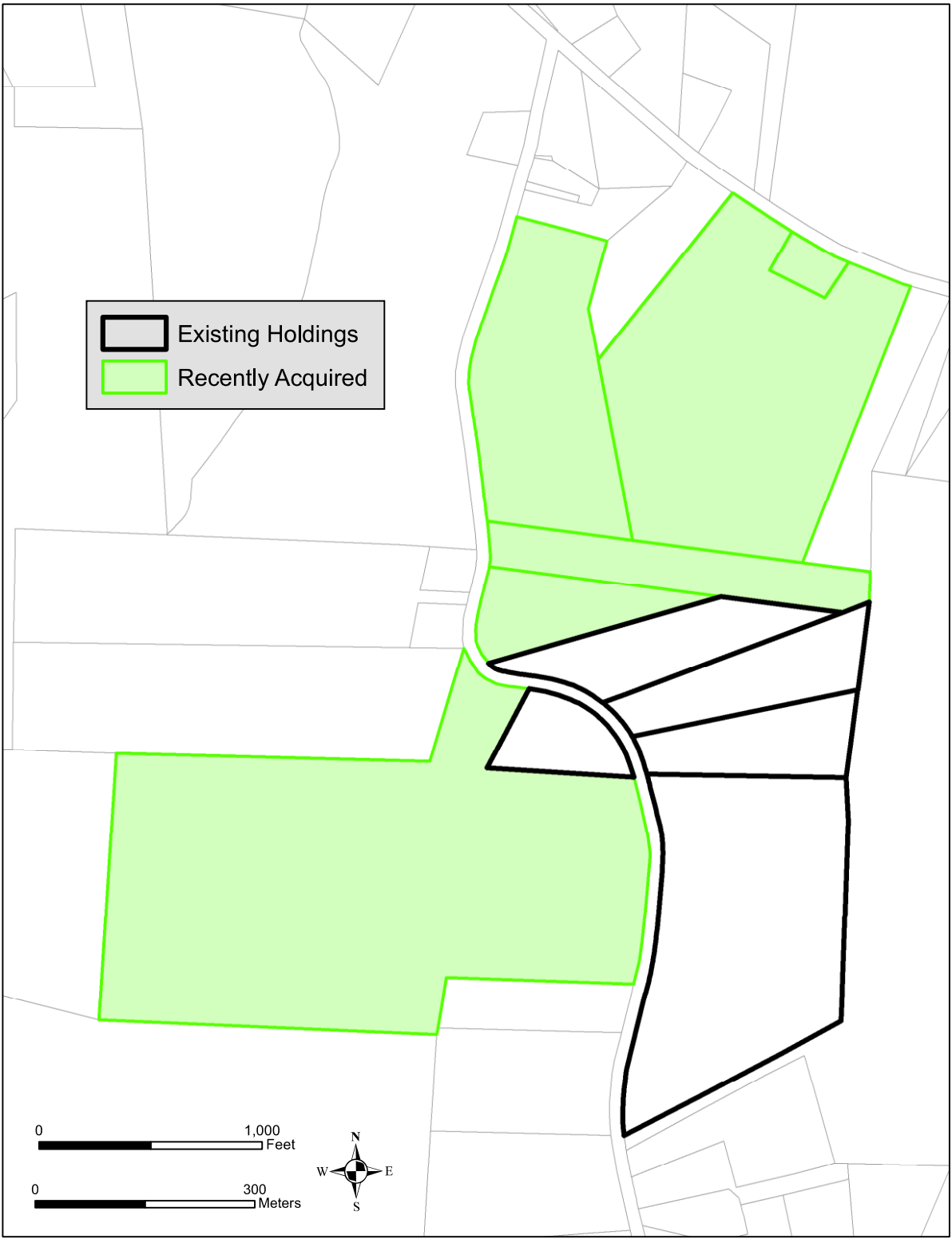
Figure 1: Map of the Group's existing and newly acquired additional mineral exploration rights at Loflin
