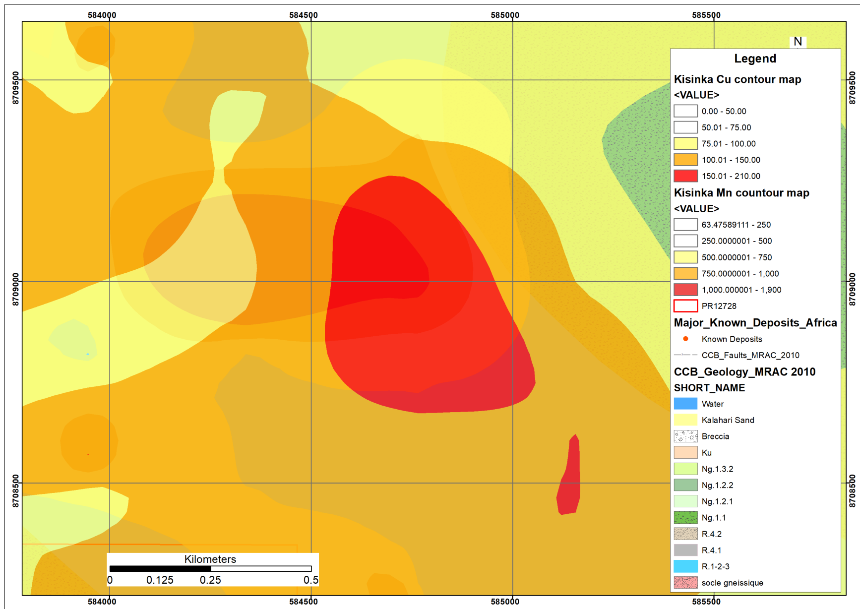
Figure 4 – Metal anomalous zone B with copper vs manganese
