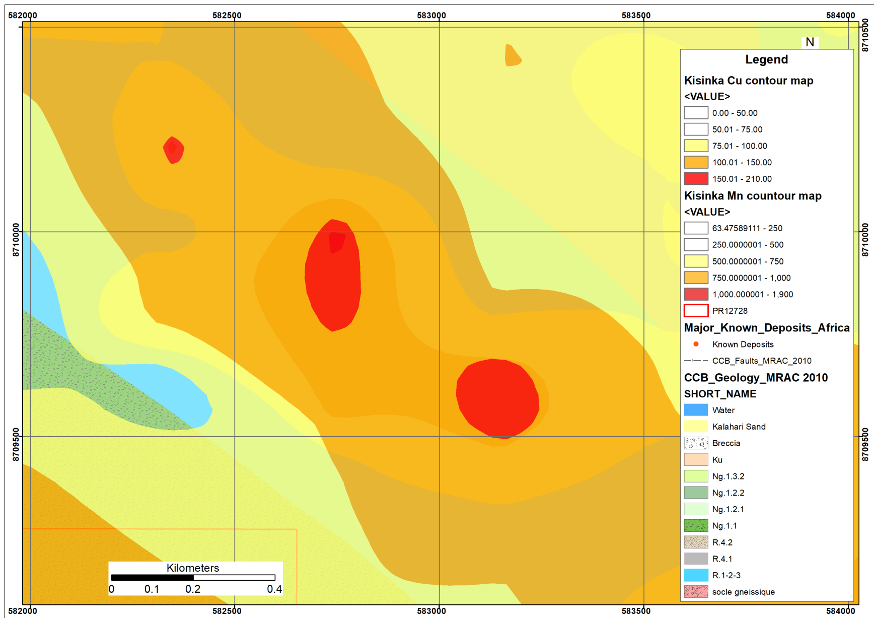
Figure 3 – Metal anomalous zone A with copper vs manganese
