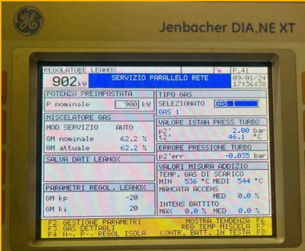
The gas engine meter indicates electricity production at 902kW, approaching the full capacity of the plant.
