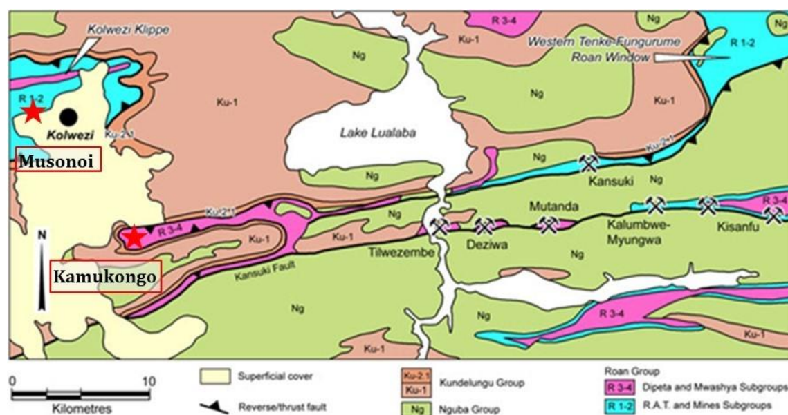
Geology of the Kansuki Fault Zone copper deposits, Katanga Province, DRC (after Gécamines)
