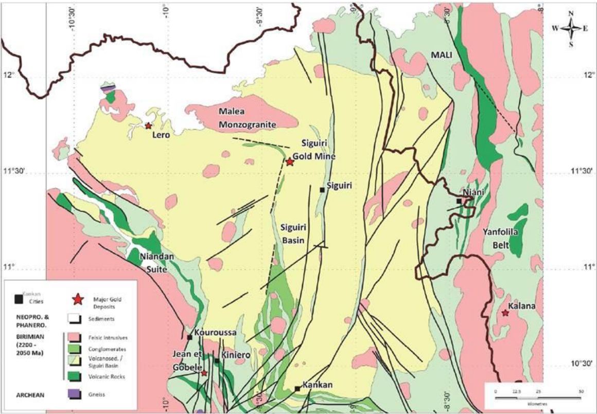
Figure 1: Location map highlighting the geology of the of Siguiri Basin with Major Gold Deposits
