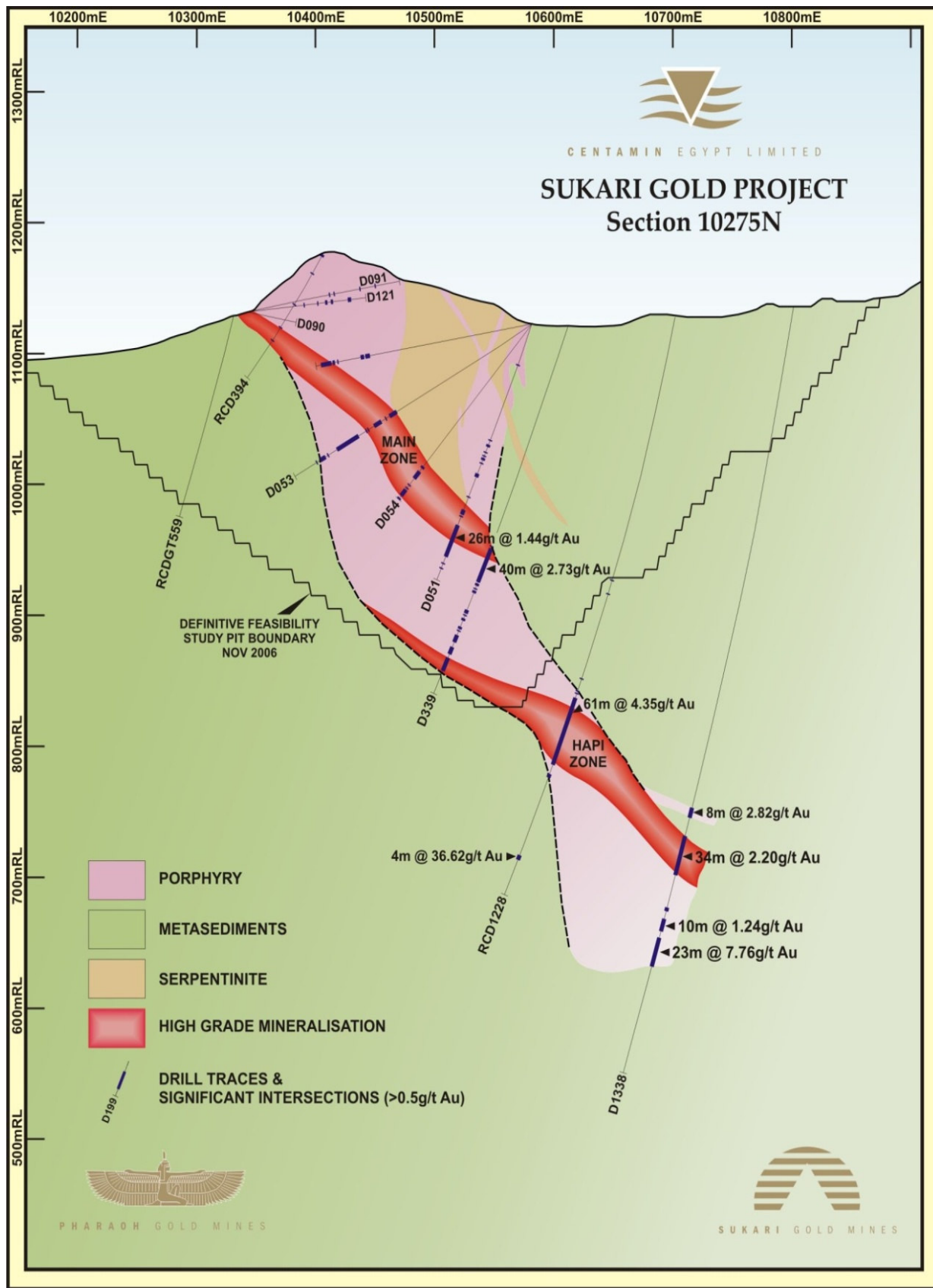
Figure 4 – Schematic Geological Section 10275N – Hole D1338
