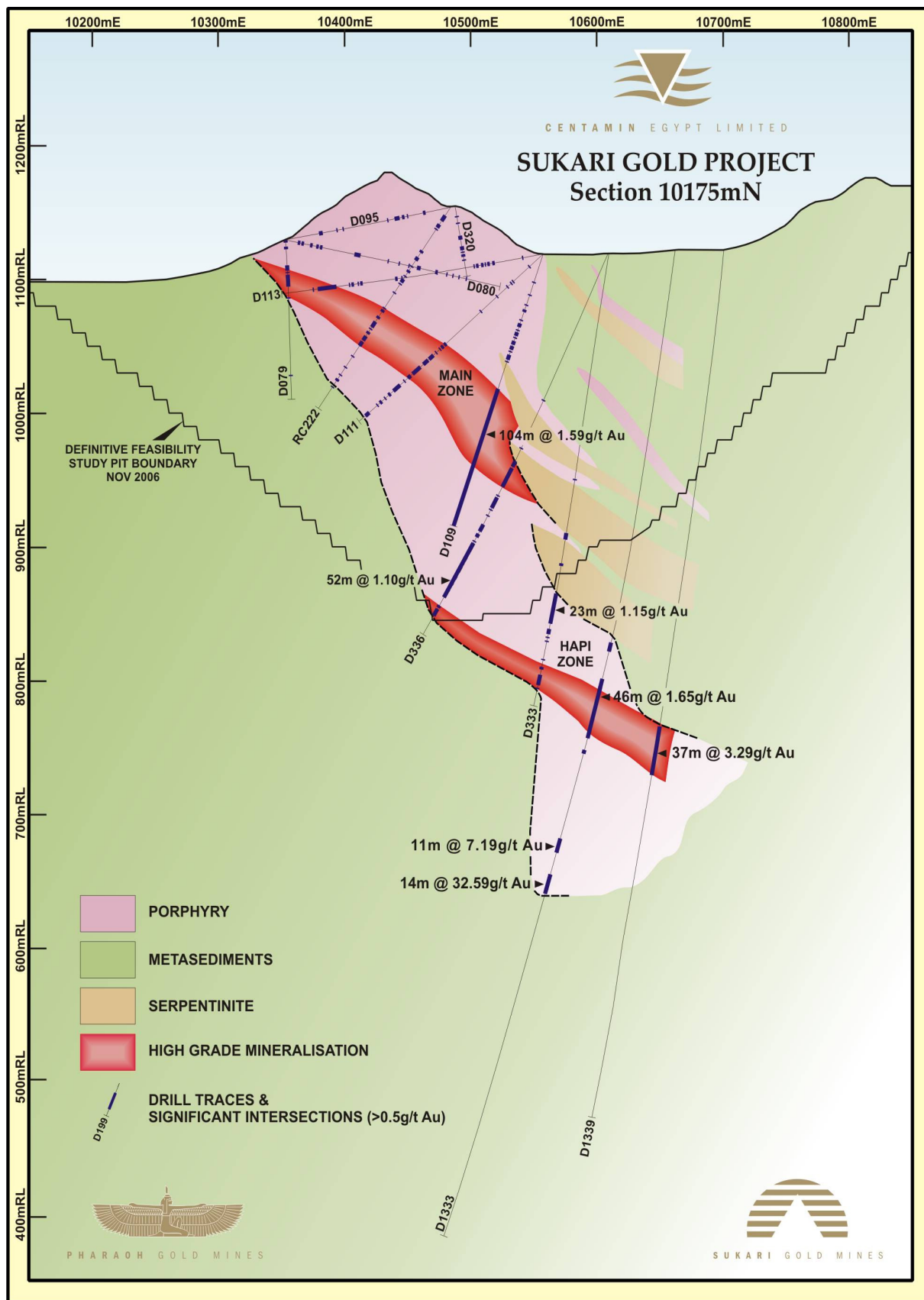
Figure 3 – Schematic Geological Section 10175N – Holes D1333 and D1339
