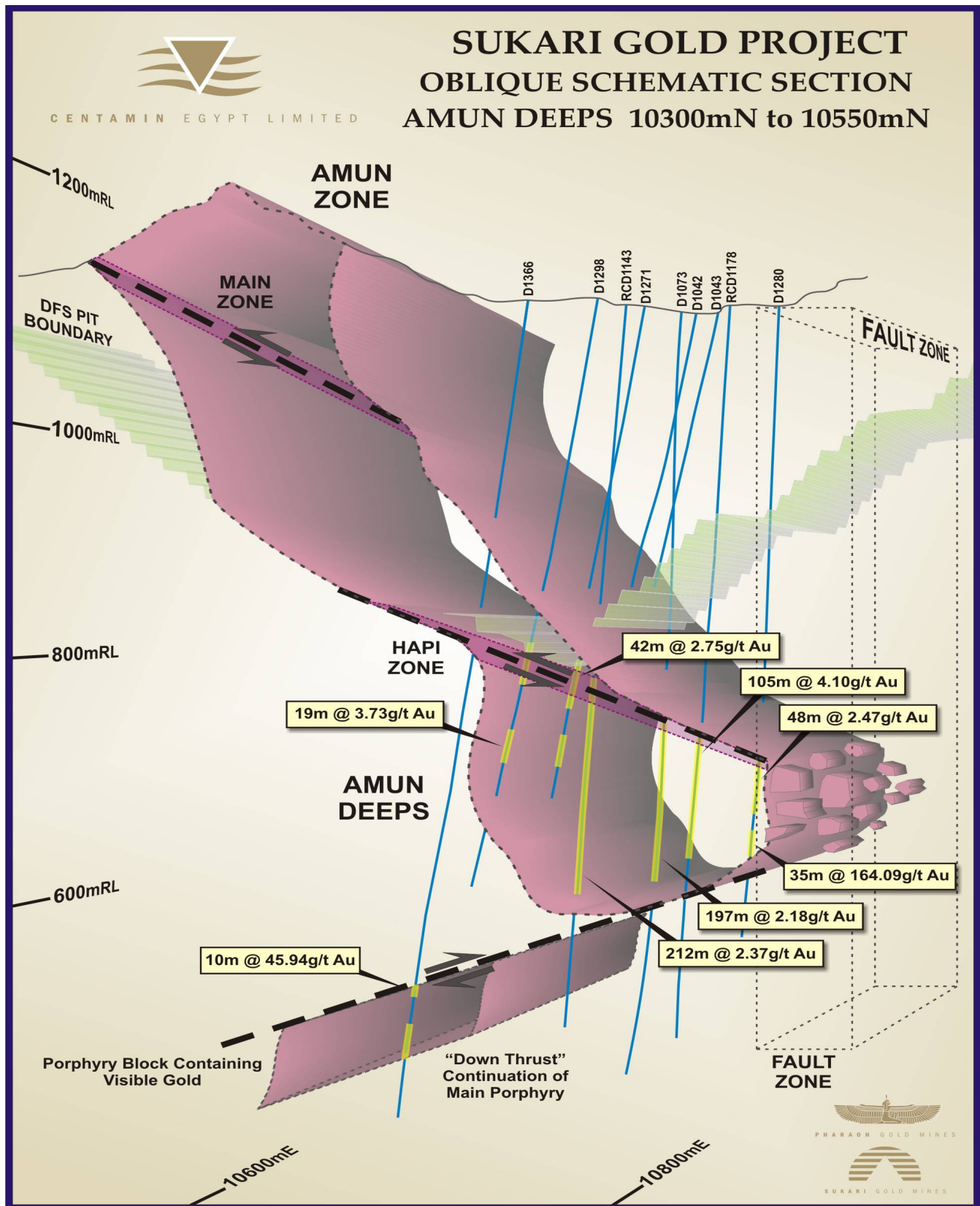
Figure 2 - Schematic Cross Section across the Amun Deeps Zone, showing main structural features, some drilling and assay intersections
