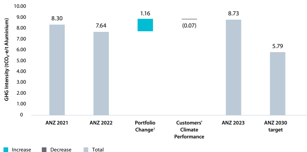
Graph 5.2 – Aluminium portfolio emissions intensity movements
