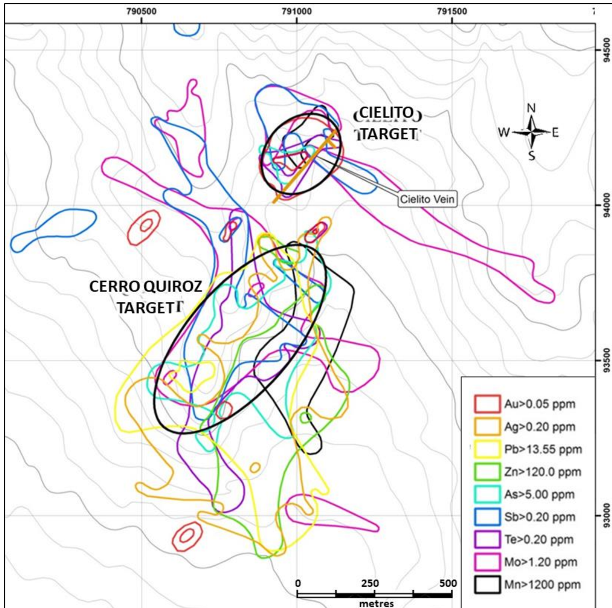
Figure 2: Plan showing the numerous co-incident soil geochemical anomalies centred upon the Cerro Quiroz dome area.
