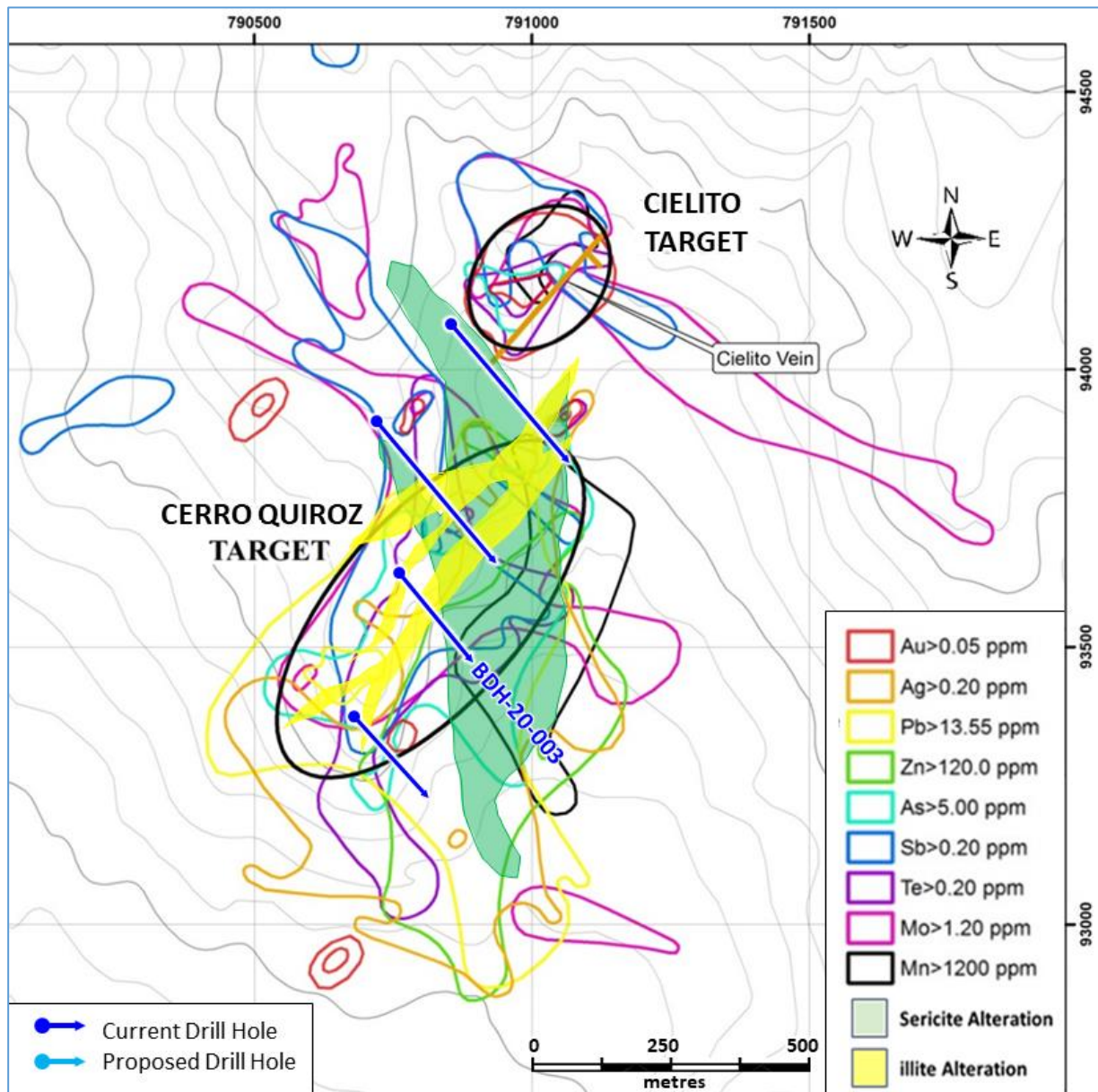
Figure 3: Plan showing the target zone at Cerro Quiroz as defined by surface geological and alteration mapping, where drill testing will target the central geochemical high and sericite-illite alteration zones.
