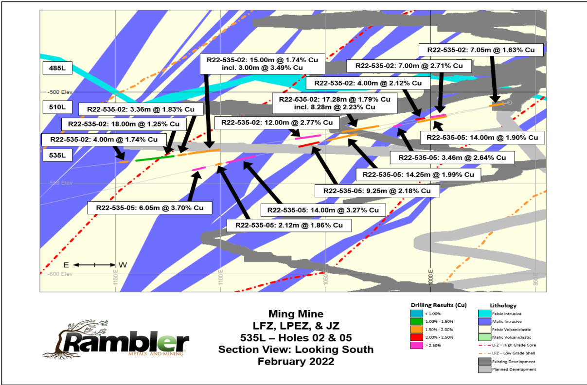
Figure 3: Section view of holes 02 and 05 from the 535L drilling program
