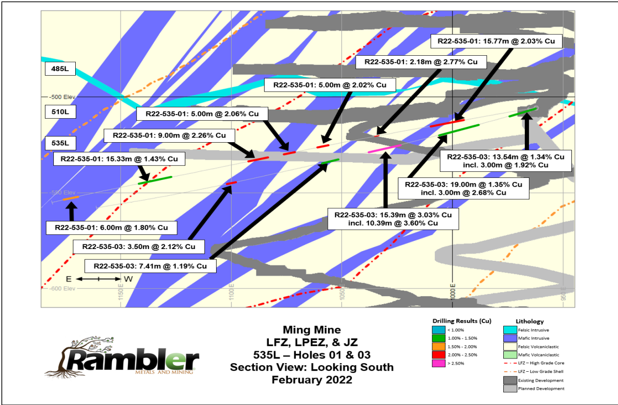
Figure 2: Section view of holes 01 and 03 from the 535L drilling program
