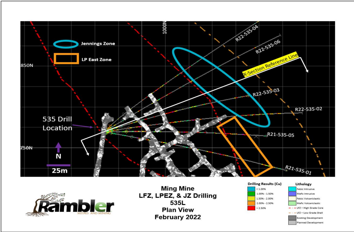
Figure 1: Plan view of LFZ, LPEZ, and JZ drilling from 535L
