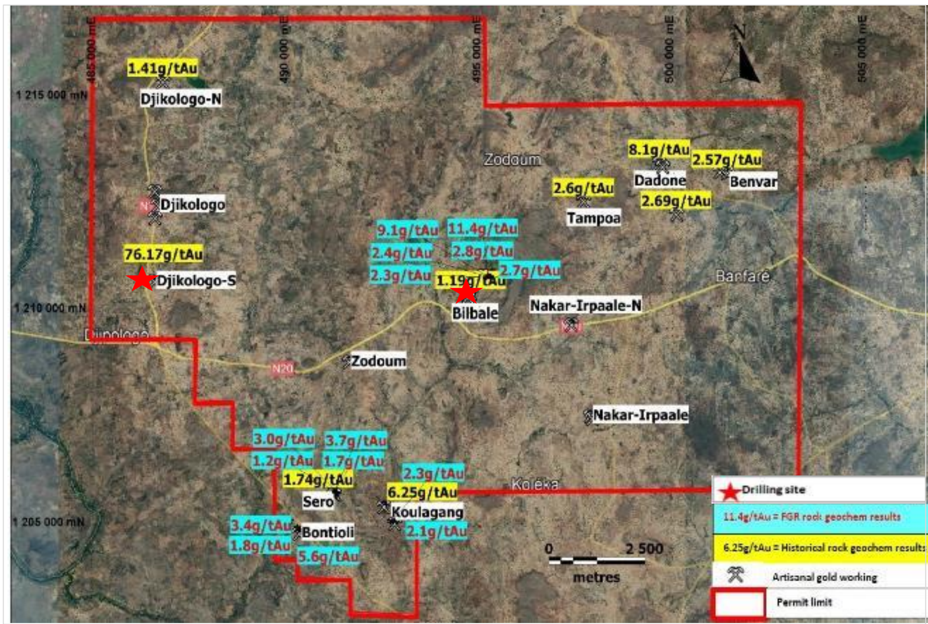
Fig 2: Rock Geochemistry in the Bilbale Licence, including 2022 work, and 2022 Drilling Locations
