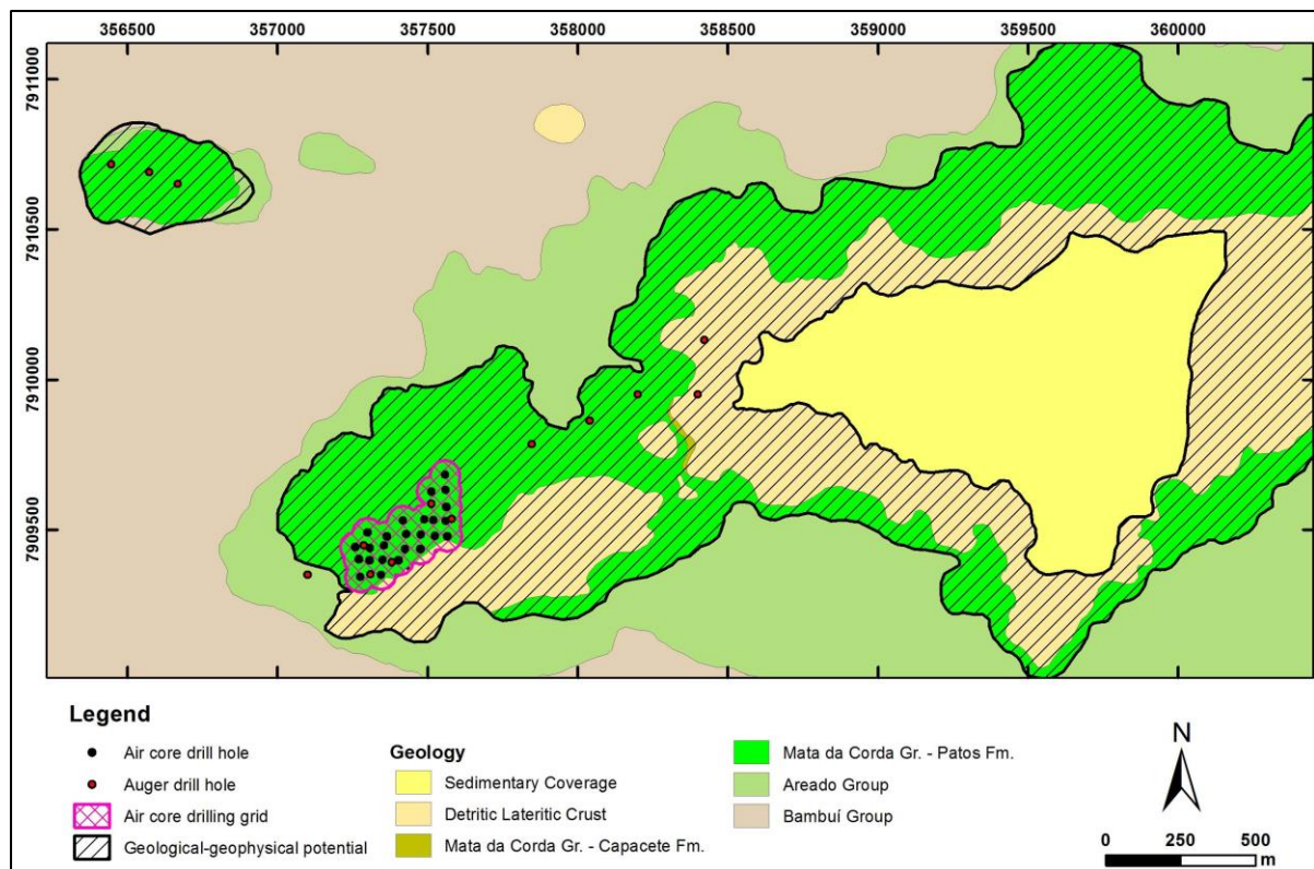
Figure 03 – Maximus Target – Exploration Potential.
