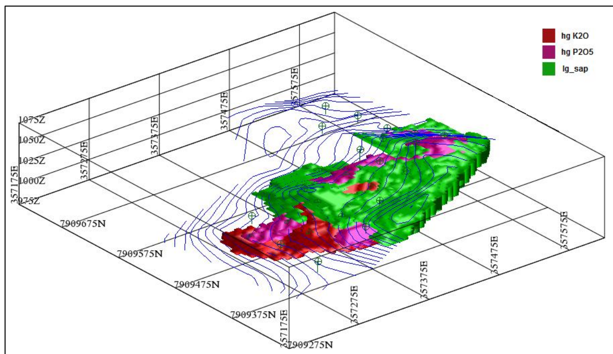
Figure 02 – Maximus Target – Block Model.
