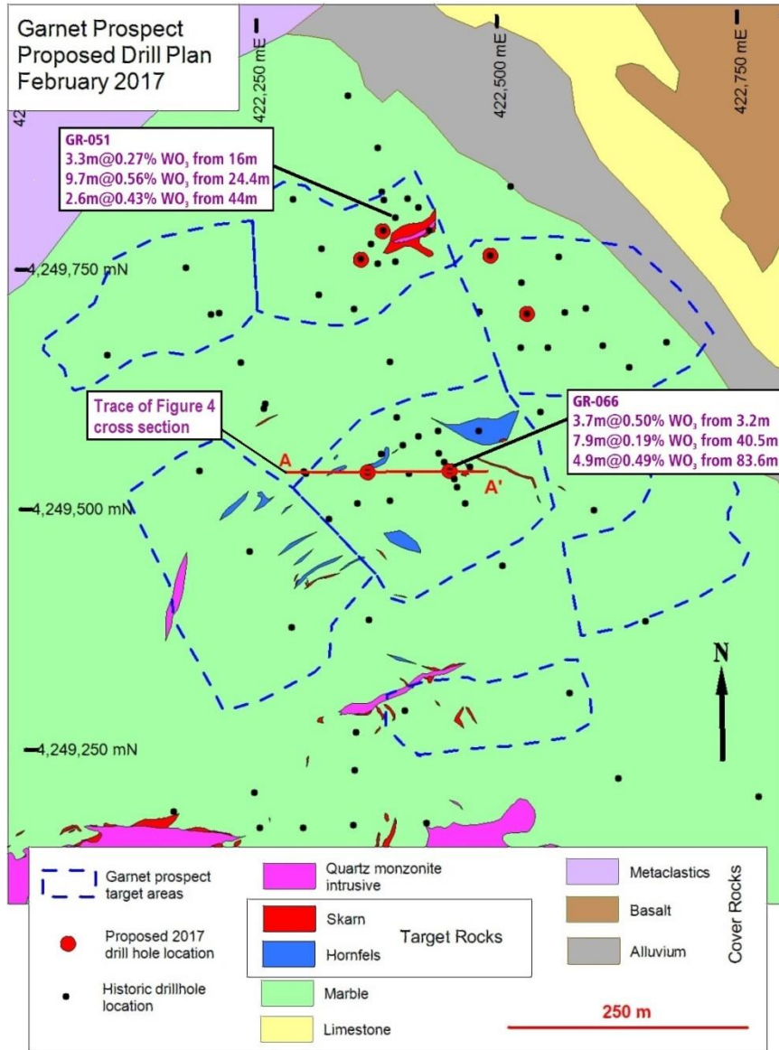
Figure 3: Six proposed RC drill holes at the Garnet prospect shown as red dots amongst historic drilling shown as black dots. The dill program will facilitate the estimation of an initial resource for the Garnet prospect.
